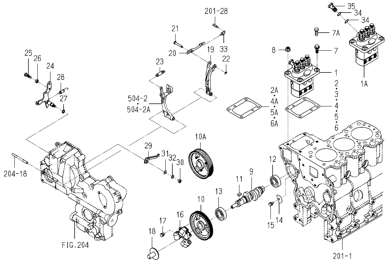
FIG.502 INJECTION PUMP
