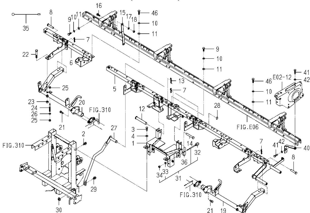
FIG.E07 FRAME(FERTILIZER)SYSTEM(1/2) (GF TYPE)
