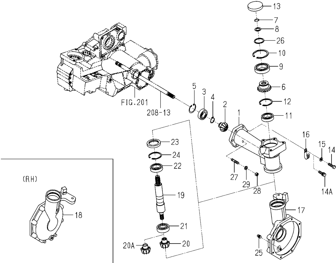
FIG.305 CASE(FINAL)SYSTEM(G TYPE)
