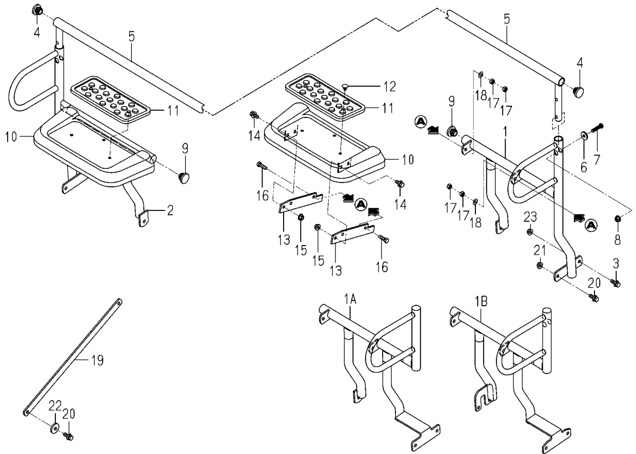
FIG.538 HANDRAIL SYSTEM(F TYPE)
