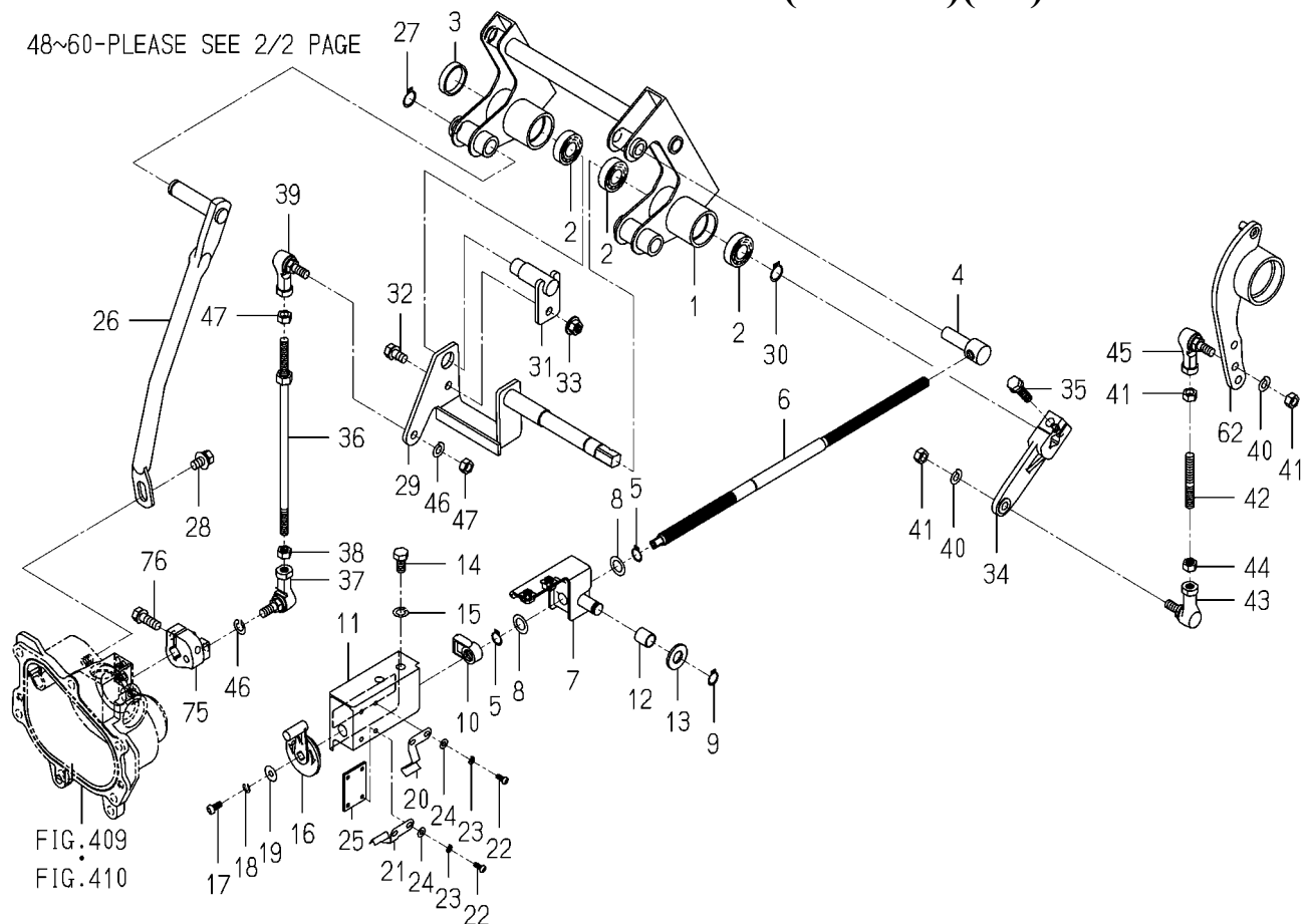
FIG.E01 DRIVE SYSTEM(F TYPE)(1/2)
