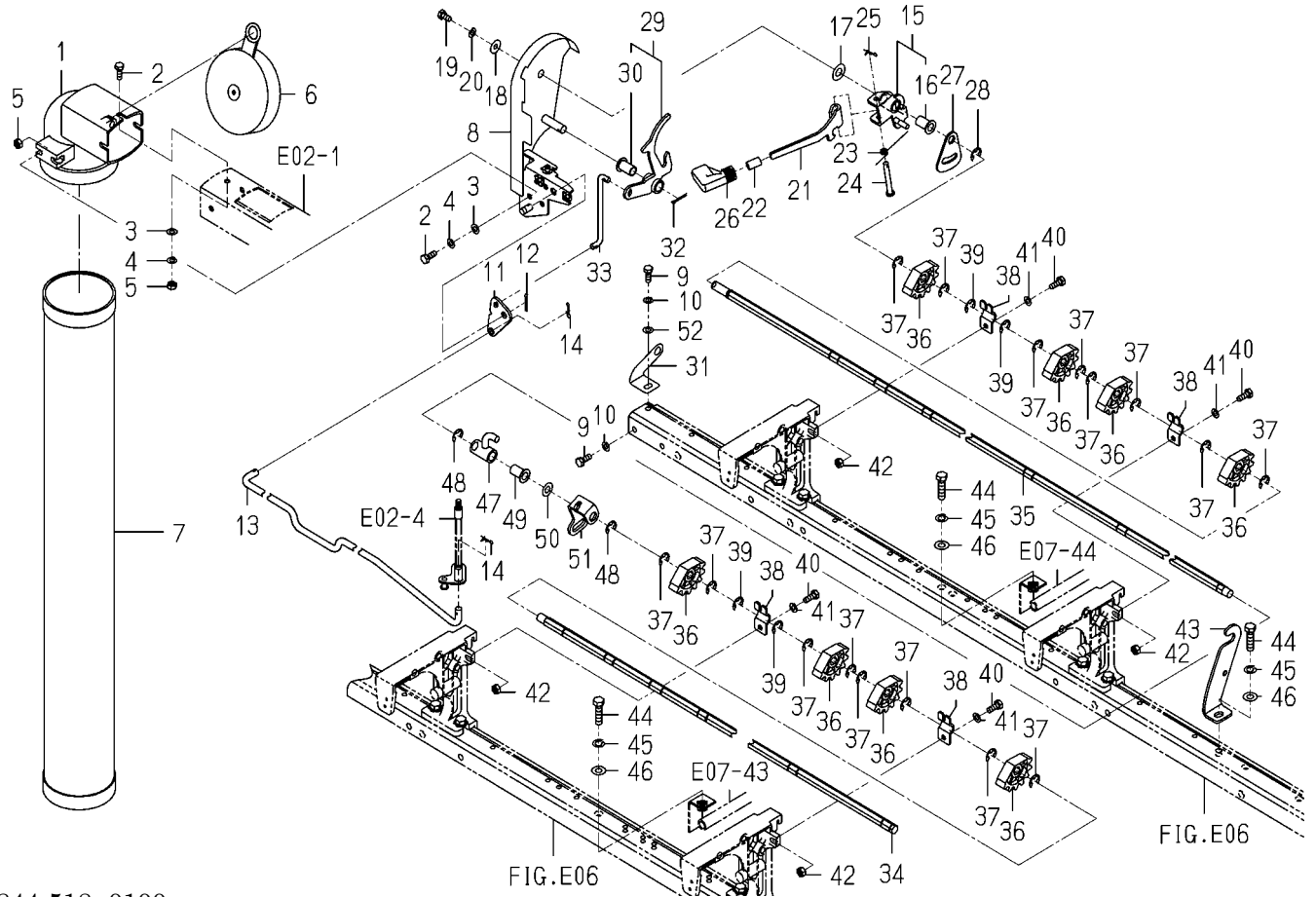
FIG.E03 DUCT(BLOW)SYSTEM(F TYPE)
