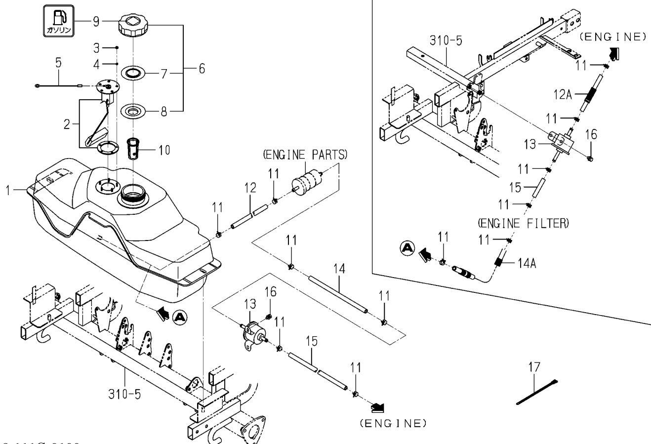
FIG.112 TANK(FUEL)SYSTEM(G TYPE)
