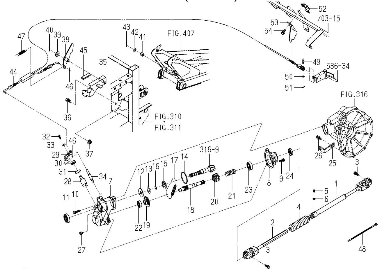
FIG.534 DRIVE(ROTOR)SYSTEM
