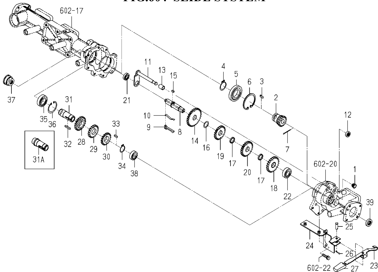
FIG.604 SLIDE SYSTEM
