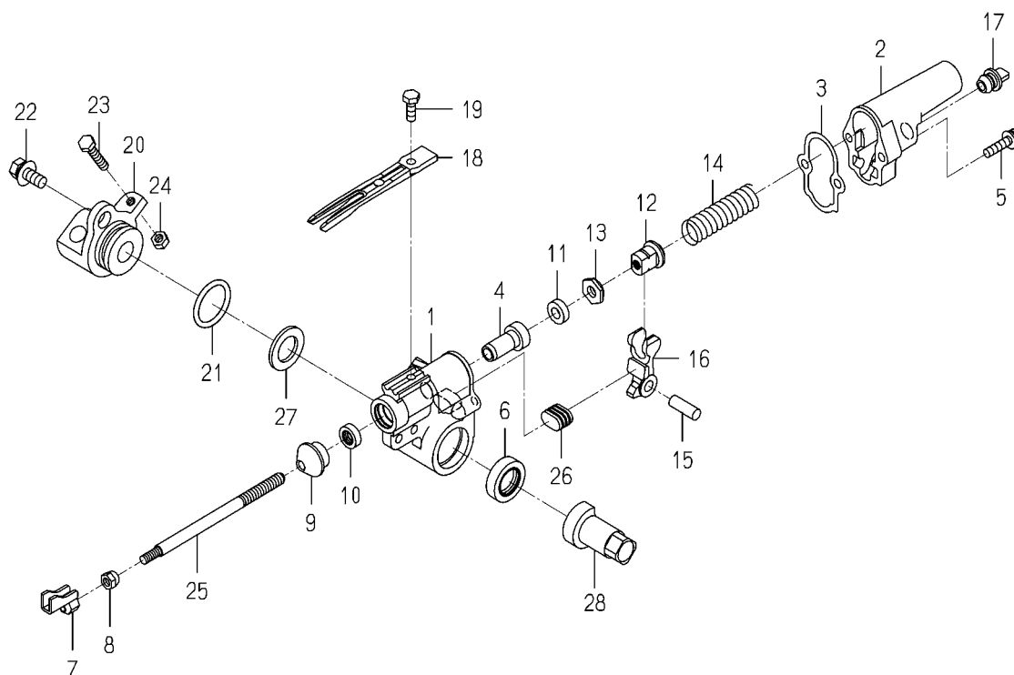
FIG.S05 COMPONENT PARTS FOR 2204-739-410-70 ON Fig.711
