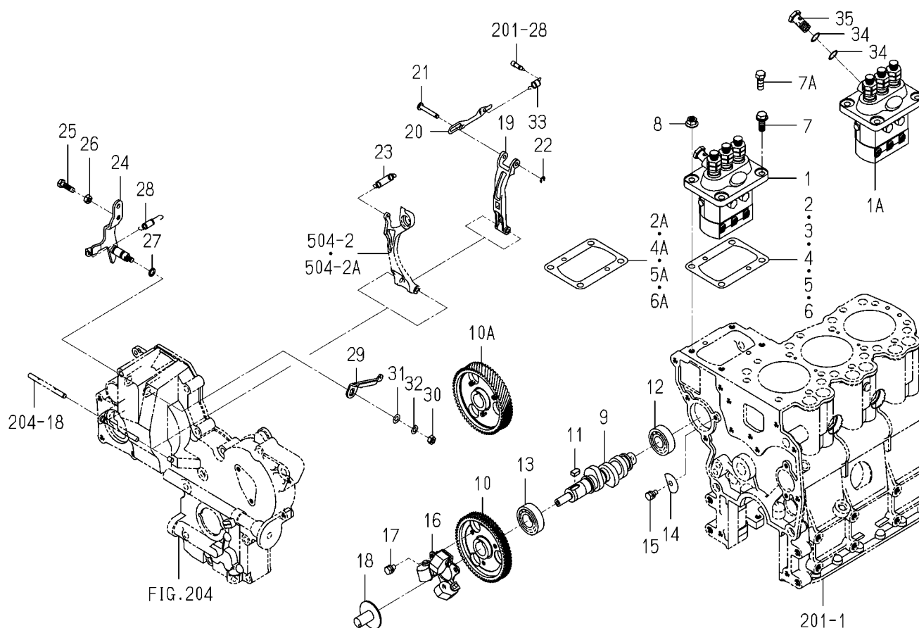
FIG.502 INJECTION PUMP
