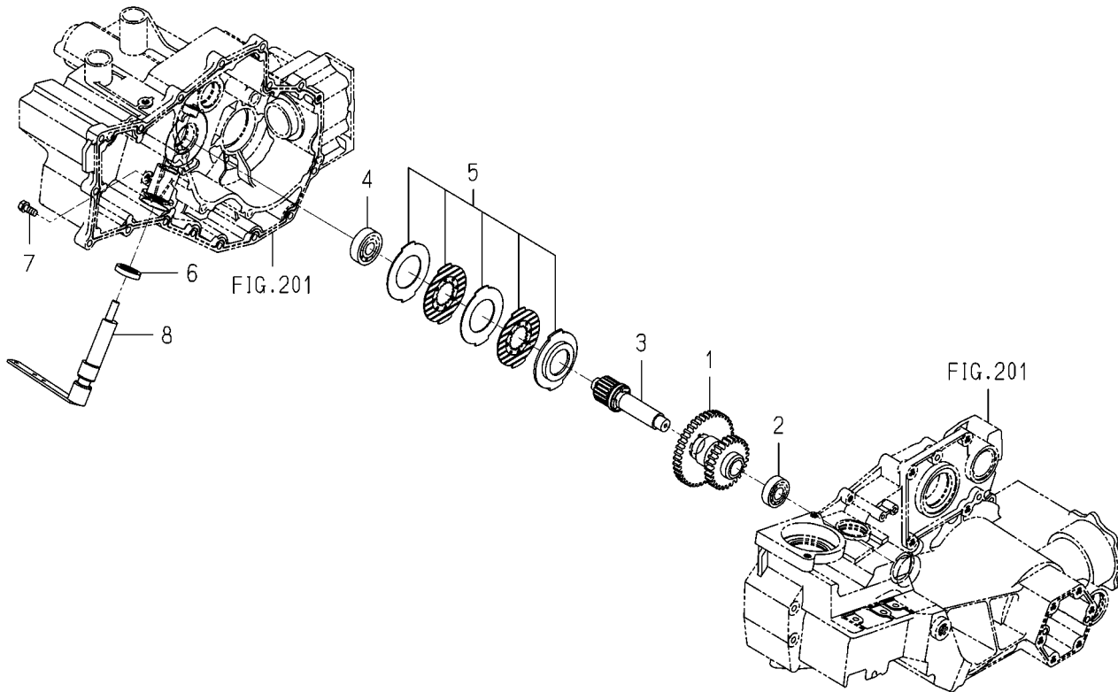
FIG.206 SHAFT(COUNTER)SYSTEM
