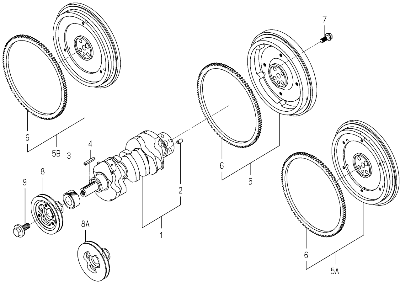
FIG.304 CRANK SHAFT
