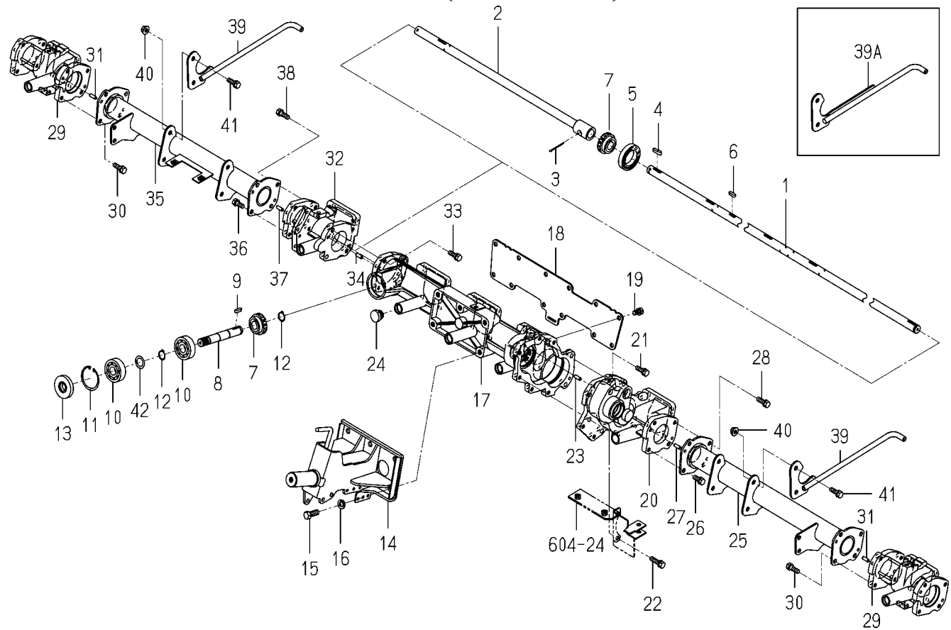
FIG.602 FRAME(PLANTING)SYSTEM
