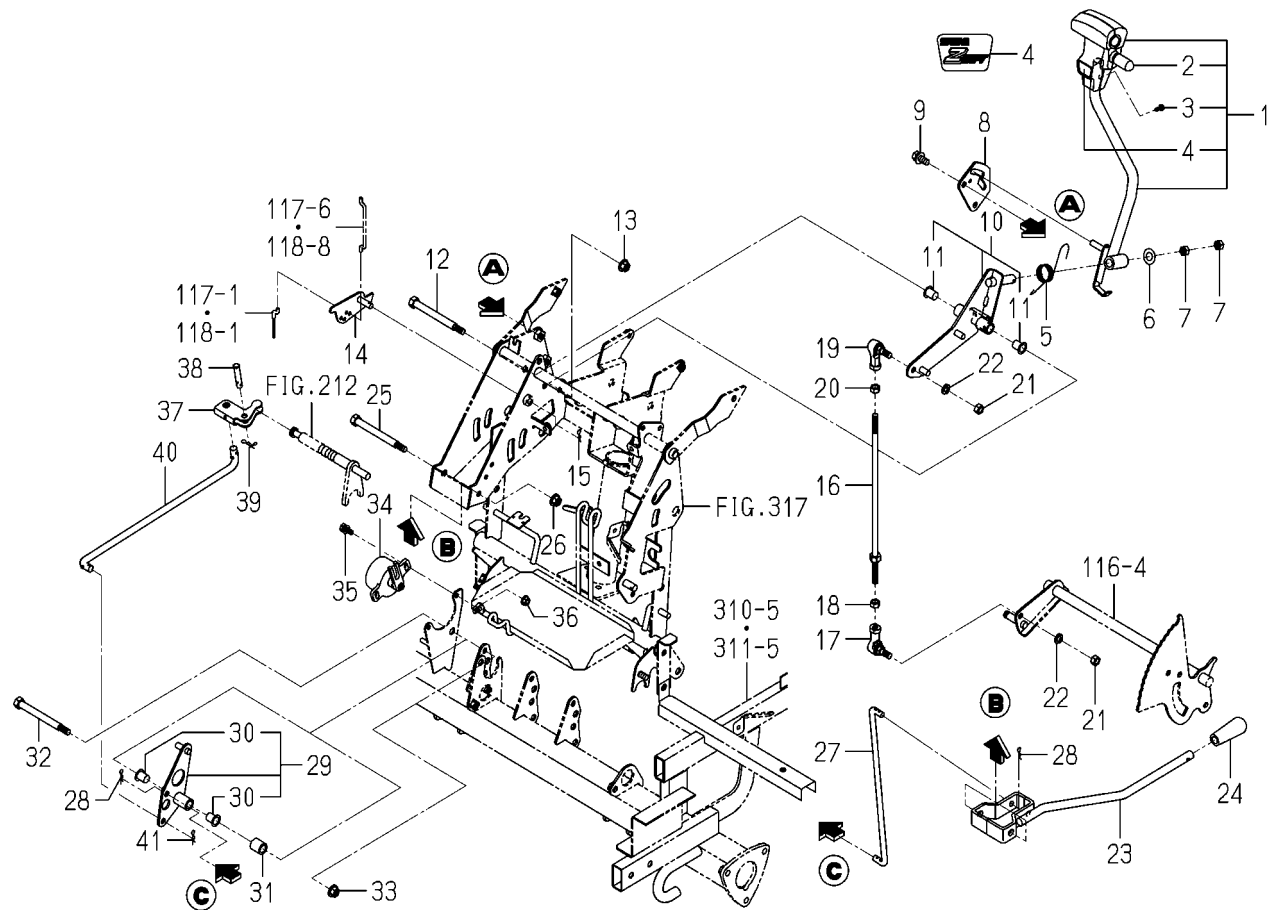
FIG.113 LEVER(HST)SYSTEM
