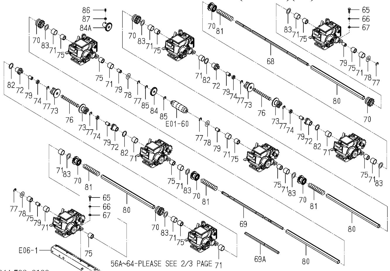
FIG.E11 OUT PUT SYSTEM(F TYPE)(3/3)
