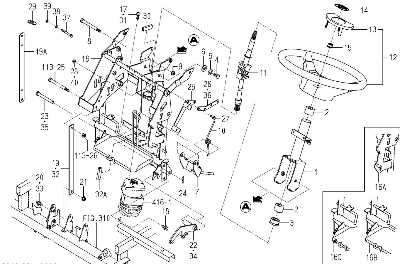
FIG.317 WHEEL(STEERING)SYSTEM
