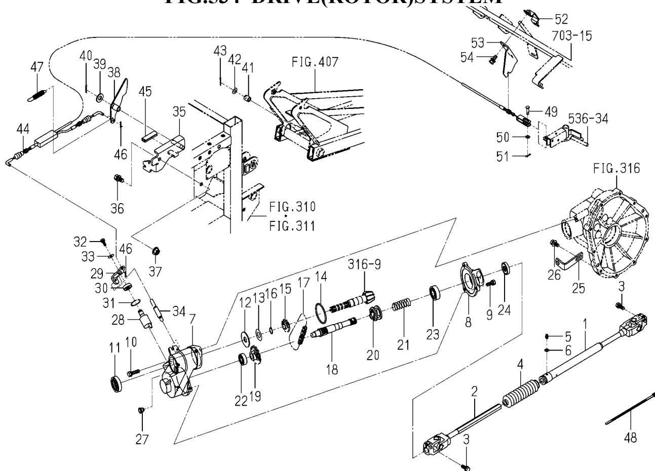
FIG.534 DRIVE(ROTOR)SYSTEM
