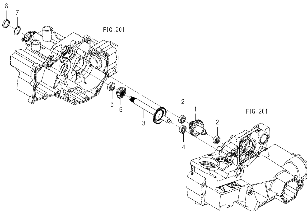
FIG.210 SHAFT(DRIVE/PLANTING)SYSTEM(G TYPE)
