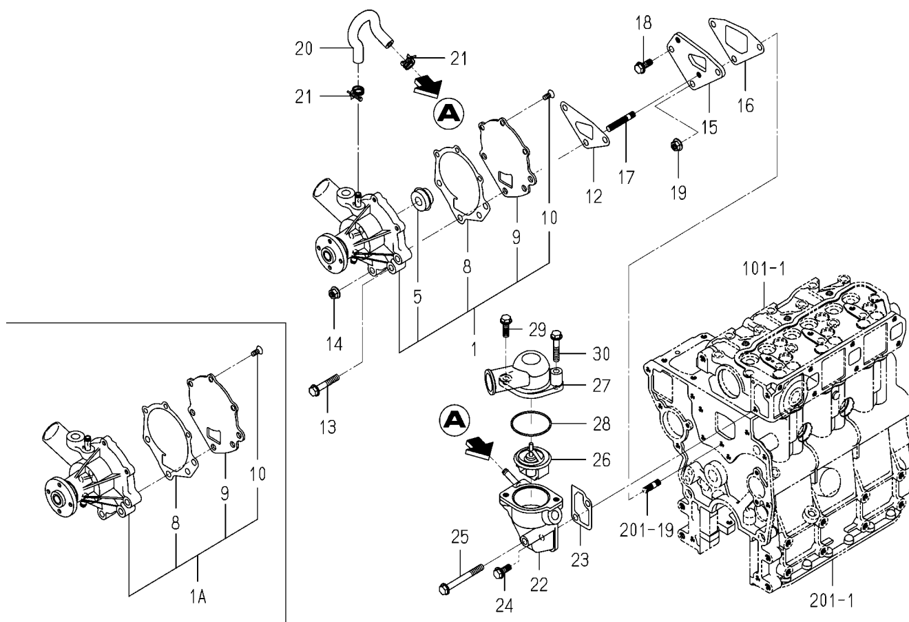
FIG.402 WATER PUMP
