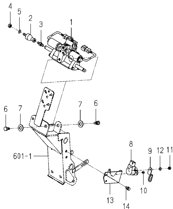
FIG.610 AUTOMATIC(ROLLING)SYSTEM
