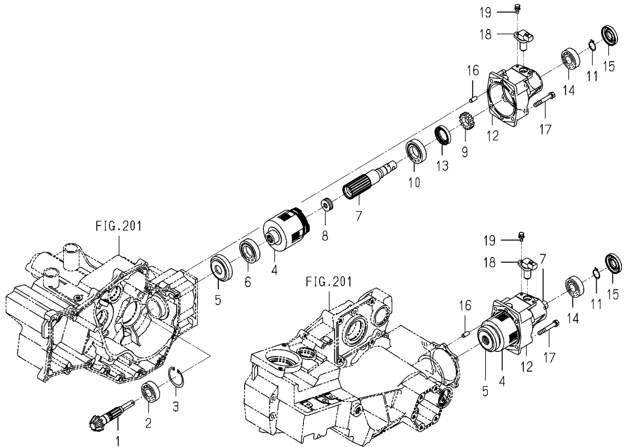
FIG.207 CLUTCH(BRAKE)SYSTEM
