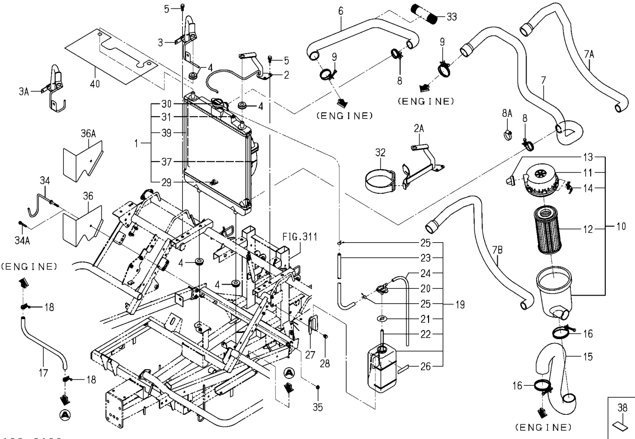
FIG.105 RADIATOR&CLEANER(AIR)SYSTEM (D TYPE)
