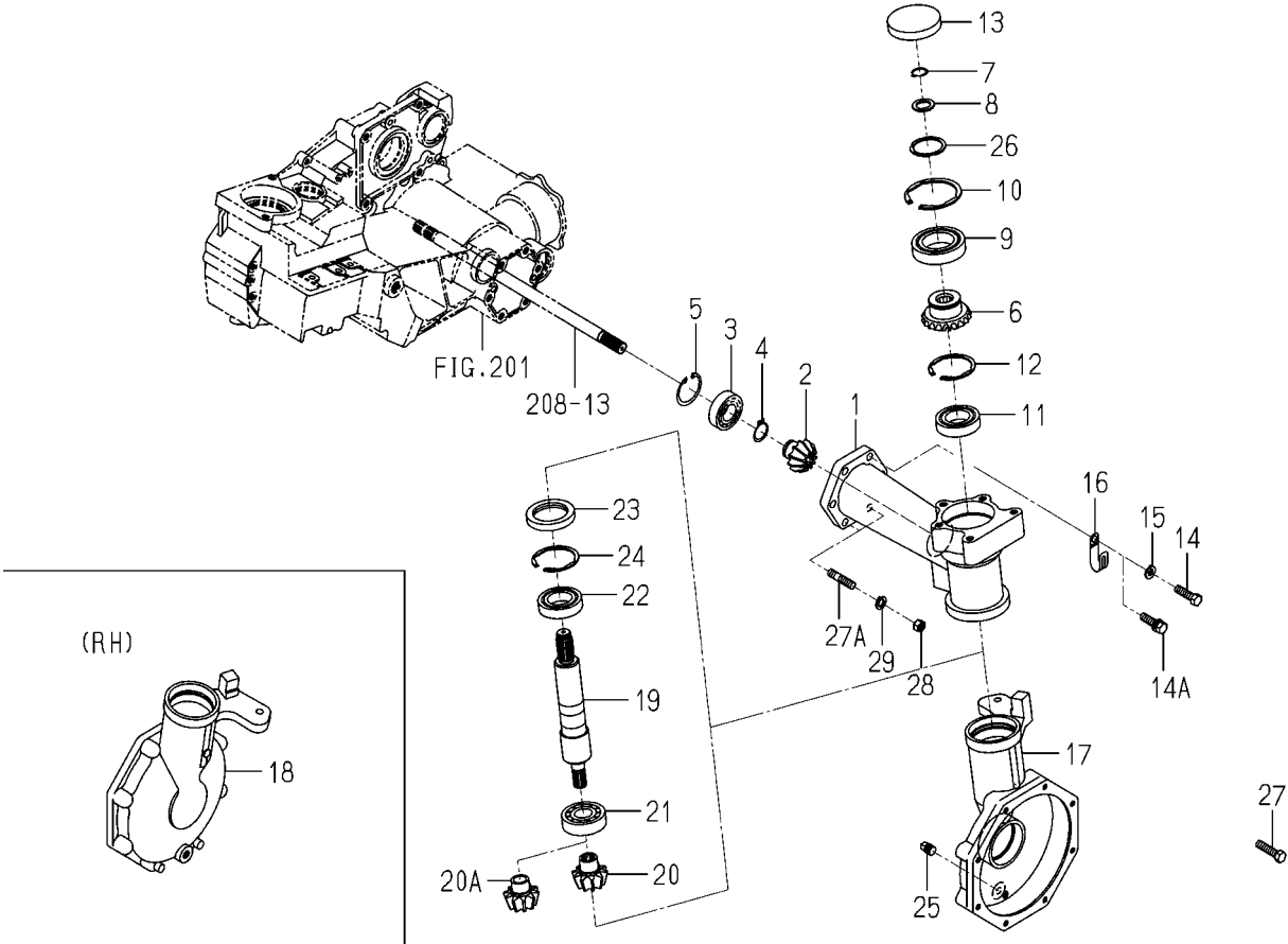
FIG.304 CASE(FINAL)SYSTEM(D TYPE)
