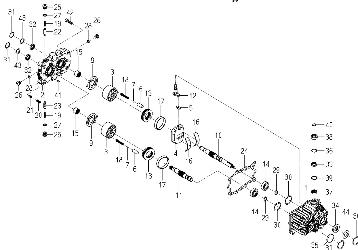
FIG.S03 COMPONENT PARTS FOR K510-019-000-20 ON Fig.114 C115
