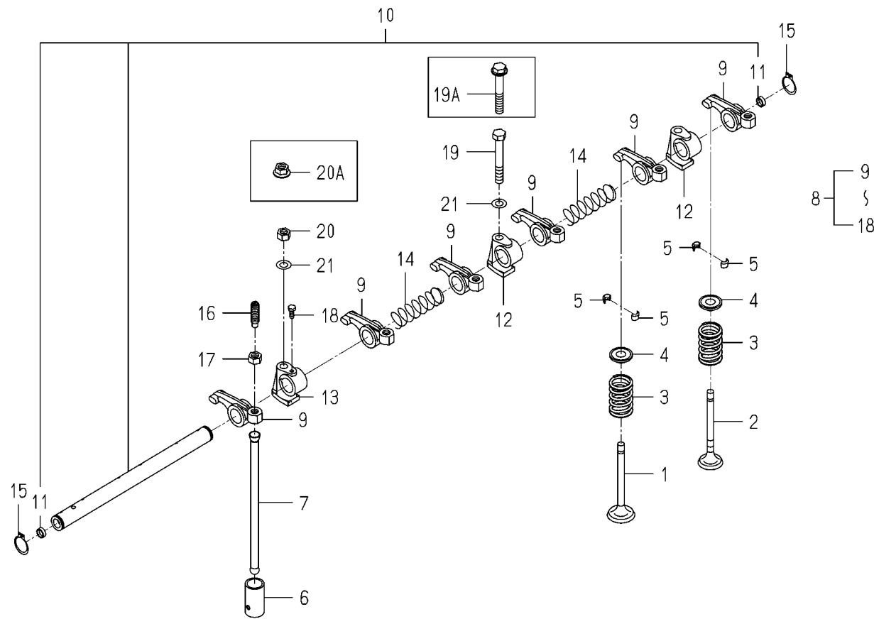
FIG.301 VALVE
