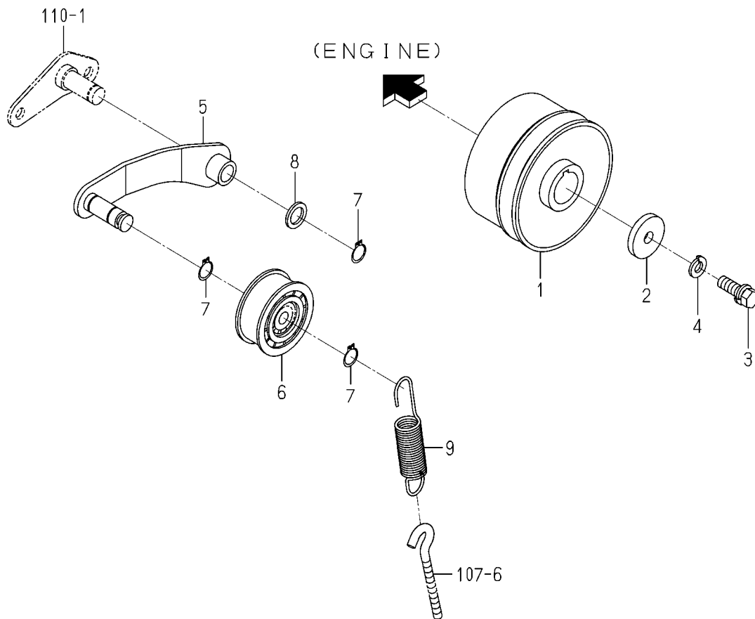
FIG.109 PULLEY(ENGINE)SYSTEM(G TYPE)
