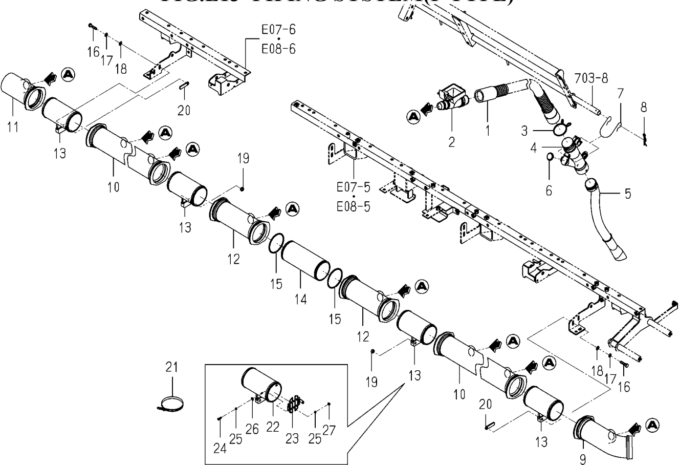
FIG.E13 PIPING SYSTEM(F TYPE)
