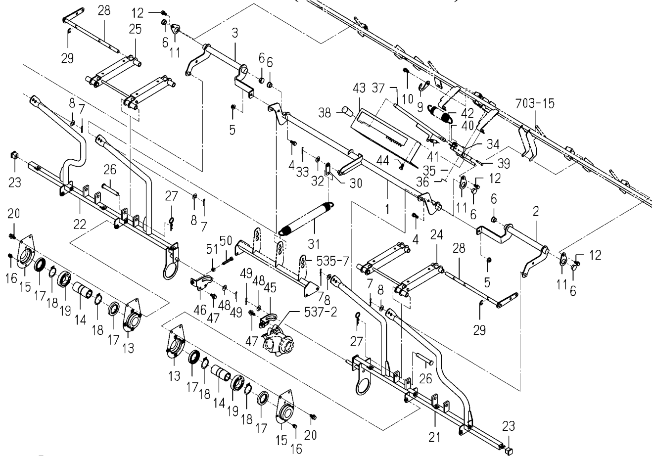
FIG.536 CONTROL(DEPTH/ROTOR)SYSTEM
