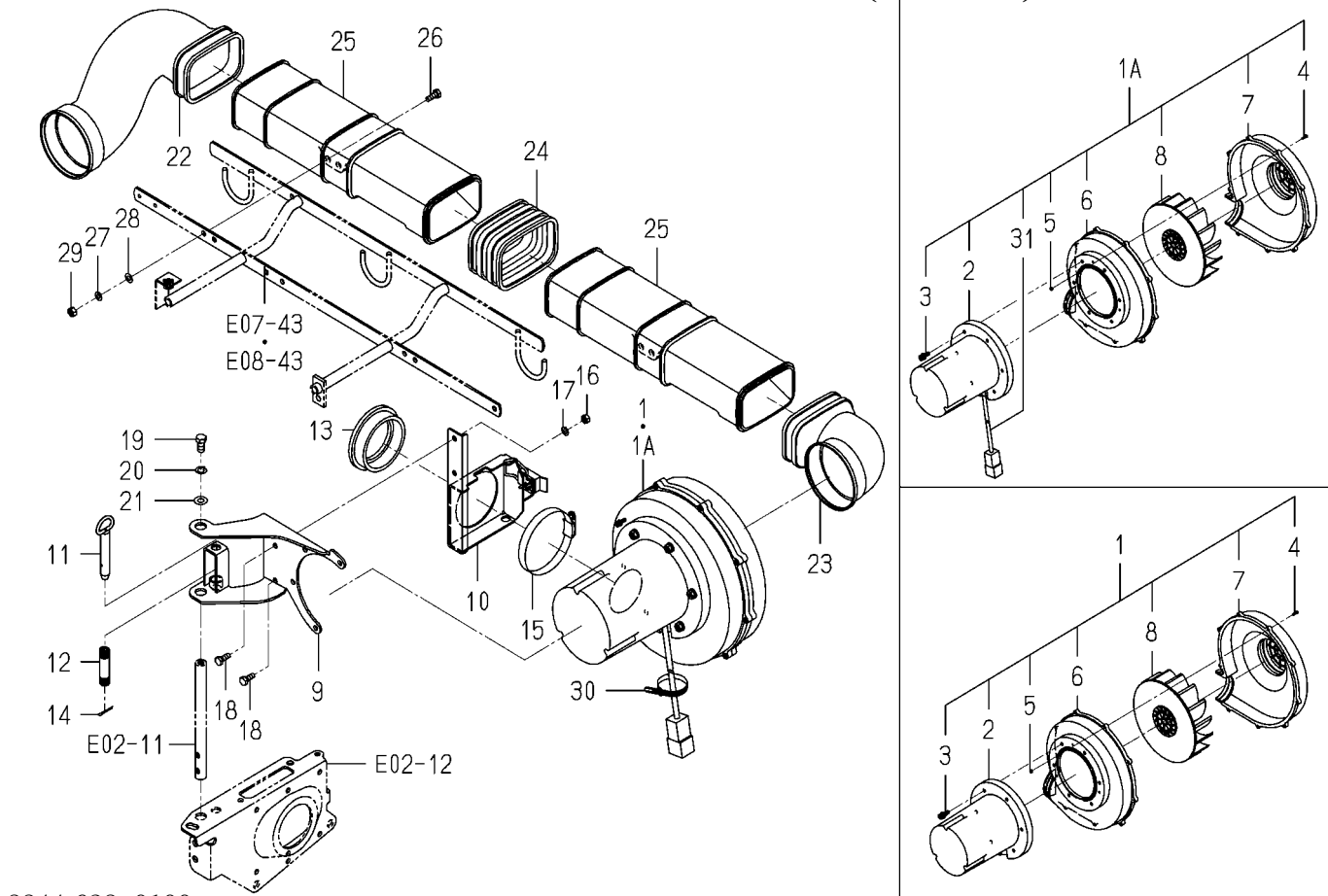
FIG.E09 BLOWER SYSTEM(F TYPE)
