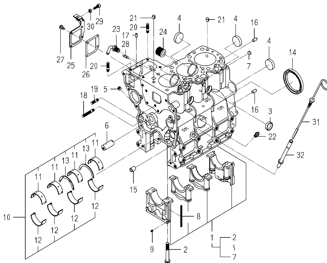
FIG.201 CYLINDER BLOCK
