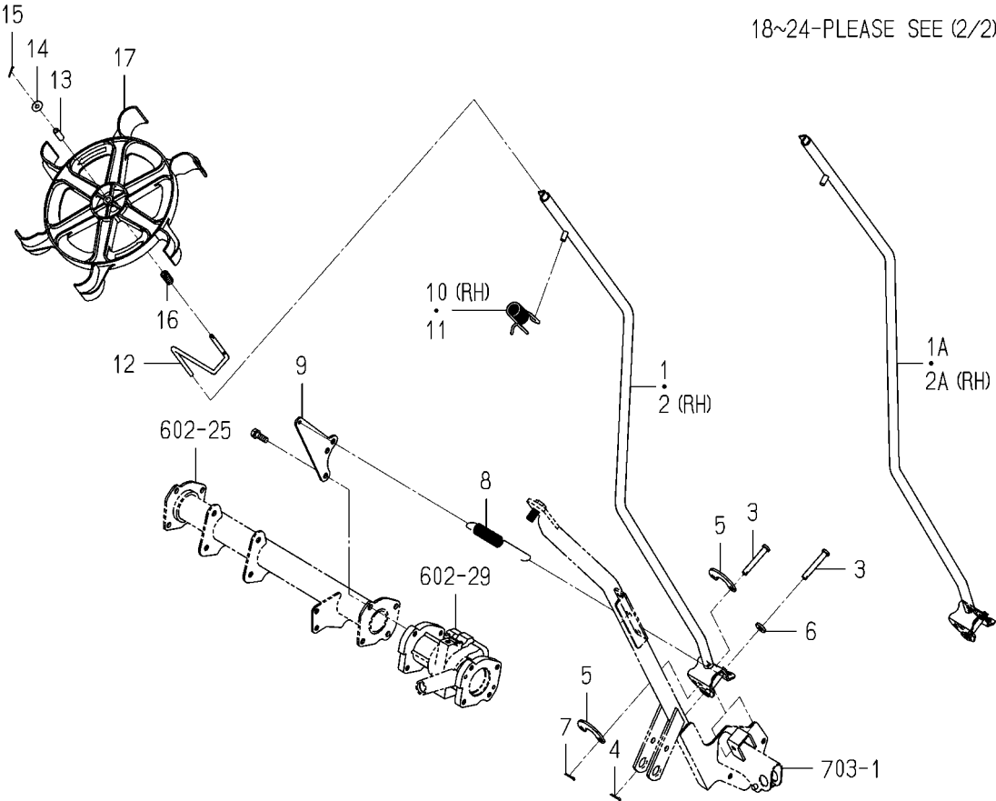
FIG.708 MARKER SYSTEM(1/2)
