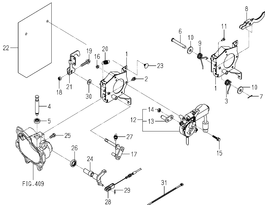
FIG.412 MOTOR(PLANTING)SYSTEM(F TYPE)
