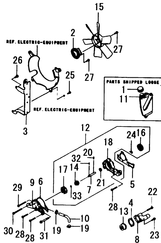
FIG. 5 COOLING-EQUIPMENT
