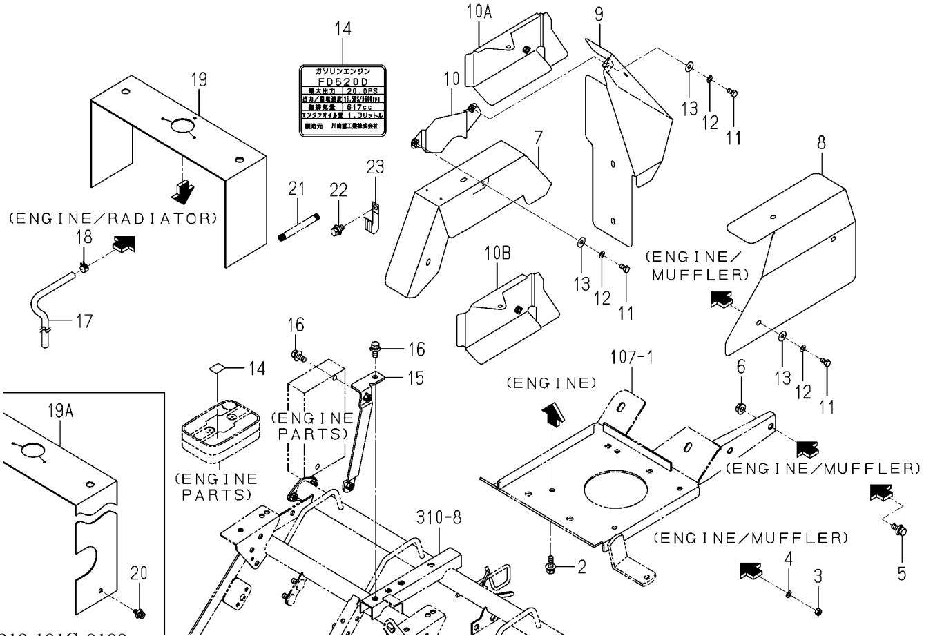
FIG.104 BRACKET(ENGINE)SYSTEM(G TYPE)
