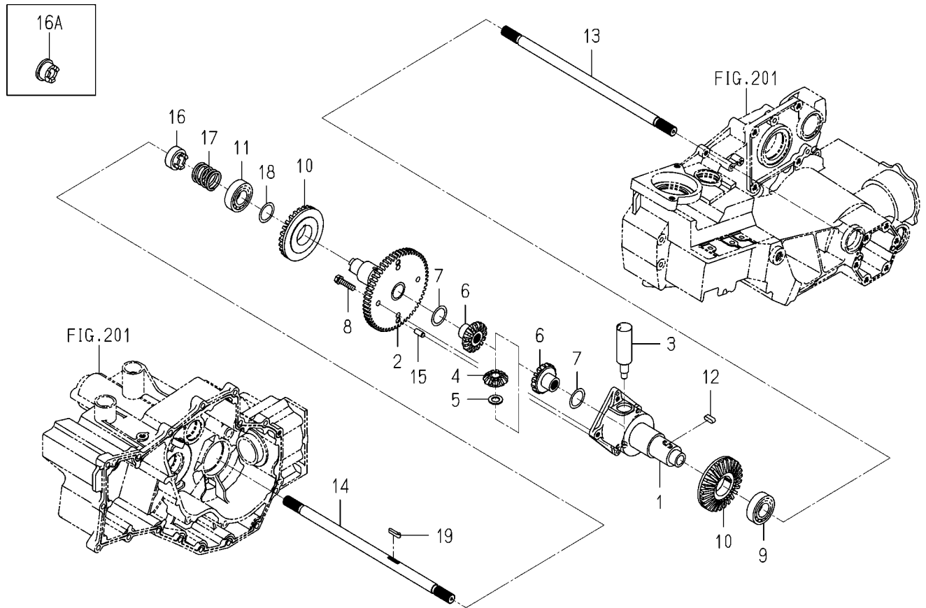
FIG.208 SHAFT(DRIVE/FRONT)SYSTEM
