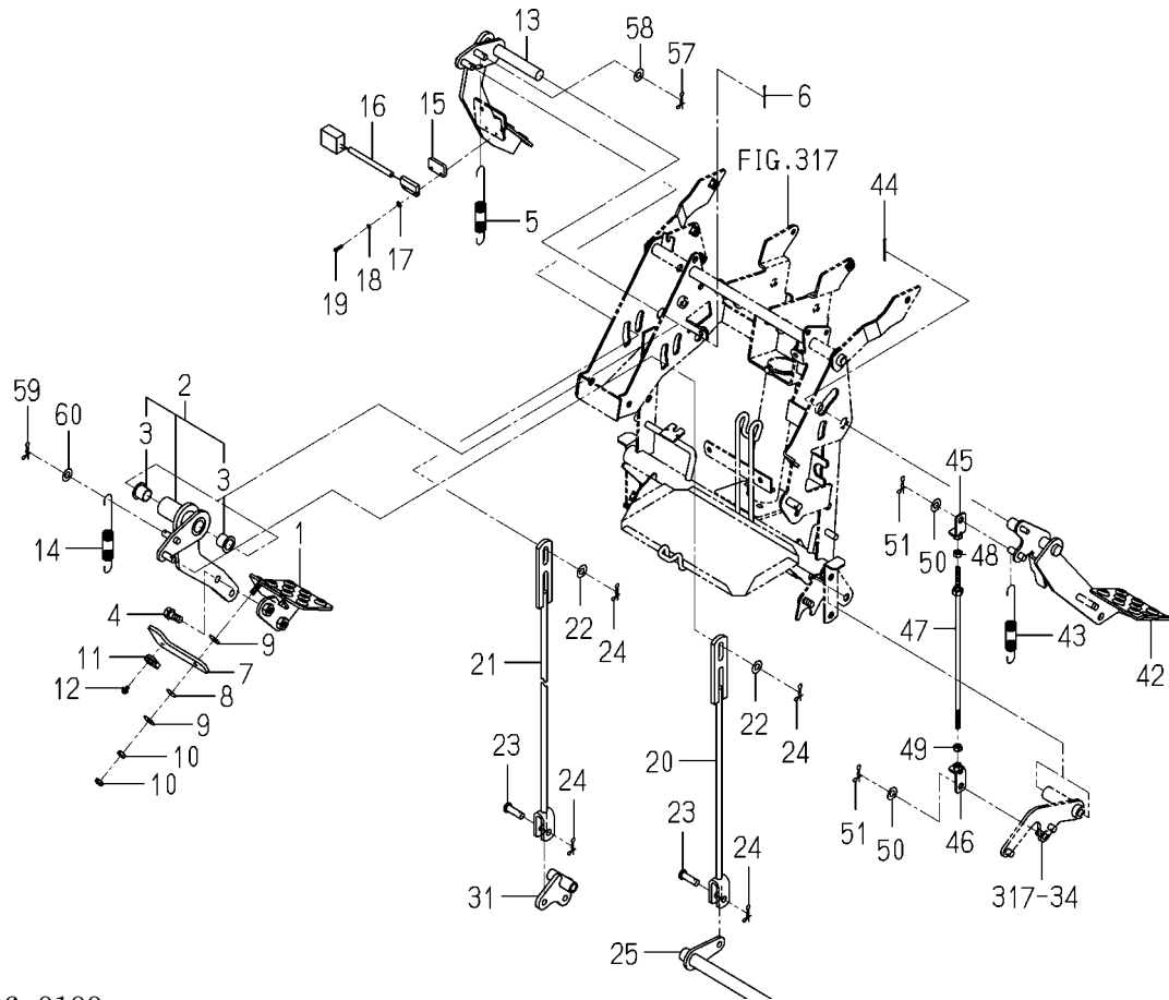
FIG.318 PEDAL SYSTEM(1/3)
