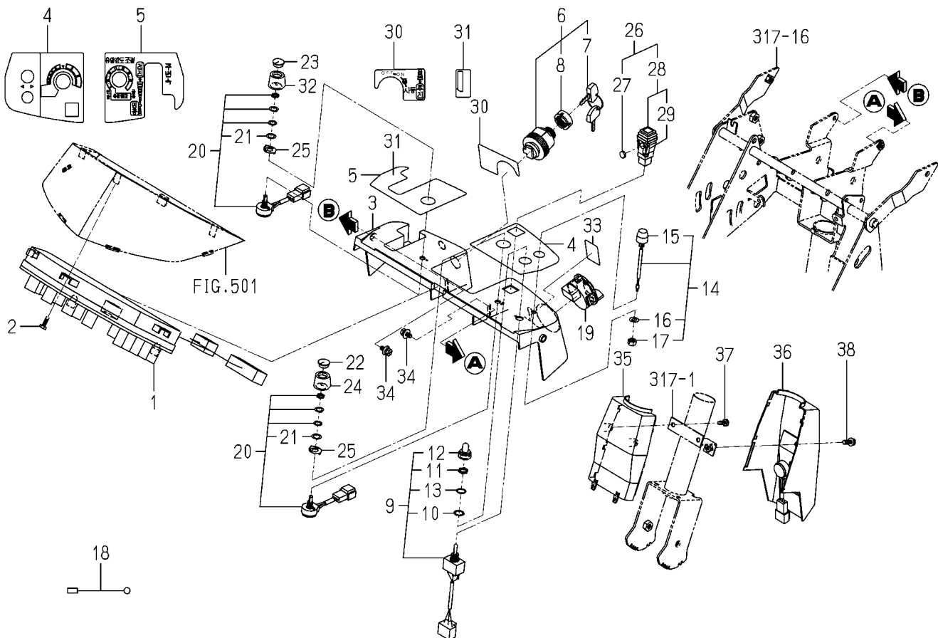
FIG.521 PANEL(MONITOR)SYSTEM(D TYPE)
