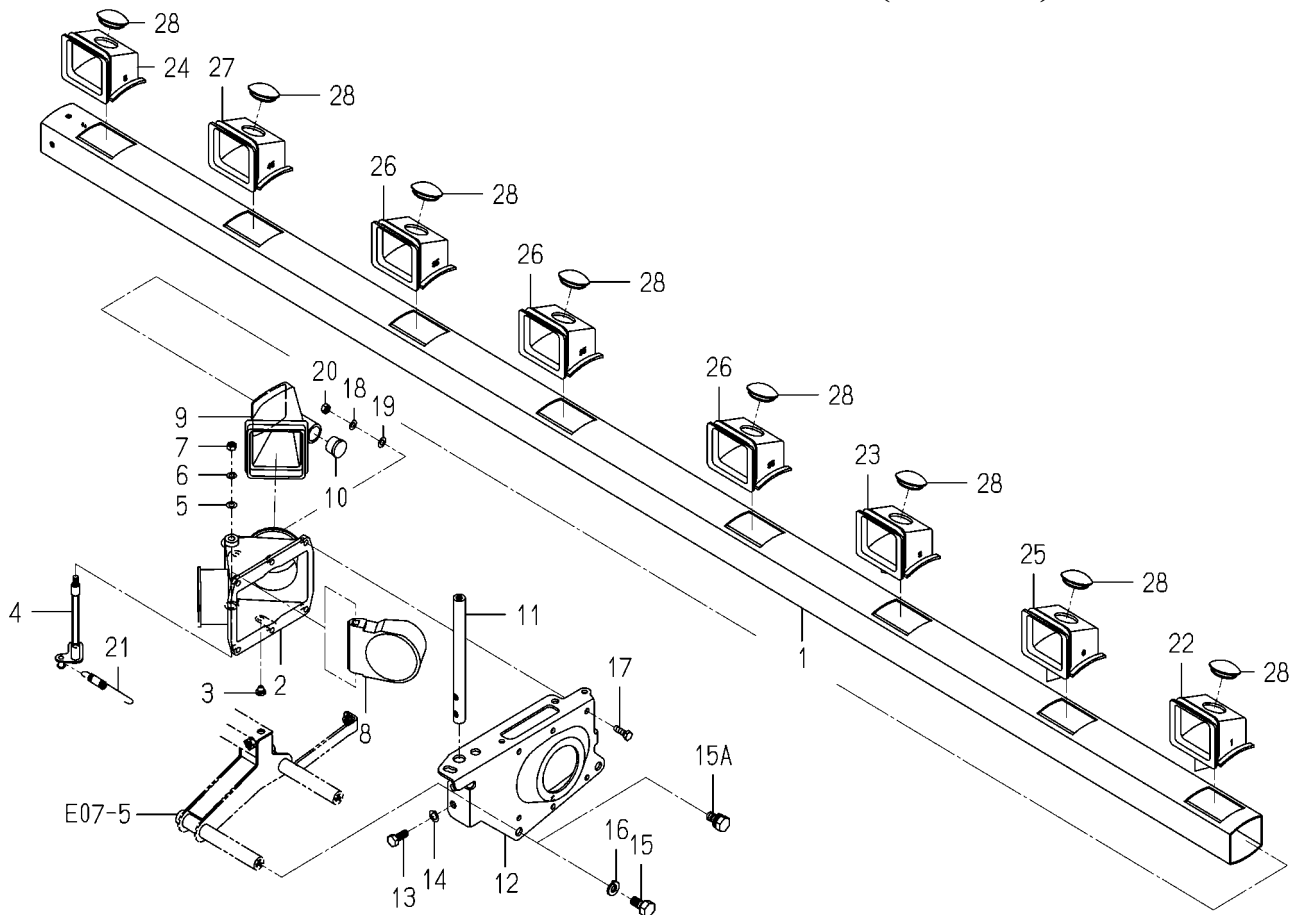
FIG.E02 AIR CHAMBER SYSTEM(F TYPE)
