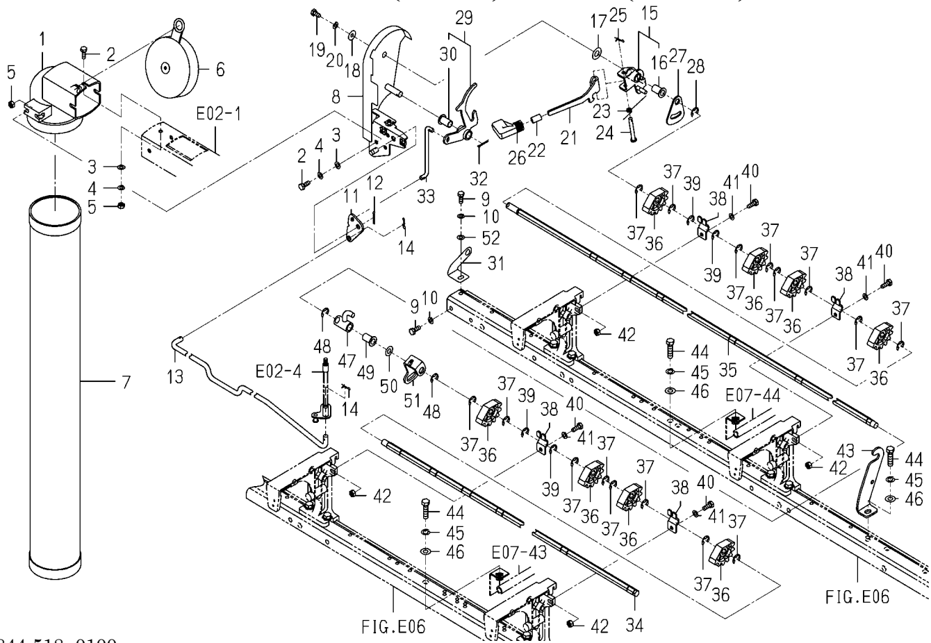
FIG.E03 DUCT(BLOW)SYSTEM(F TYPE)
