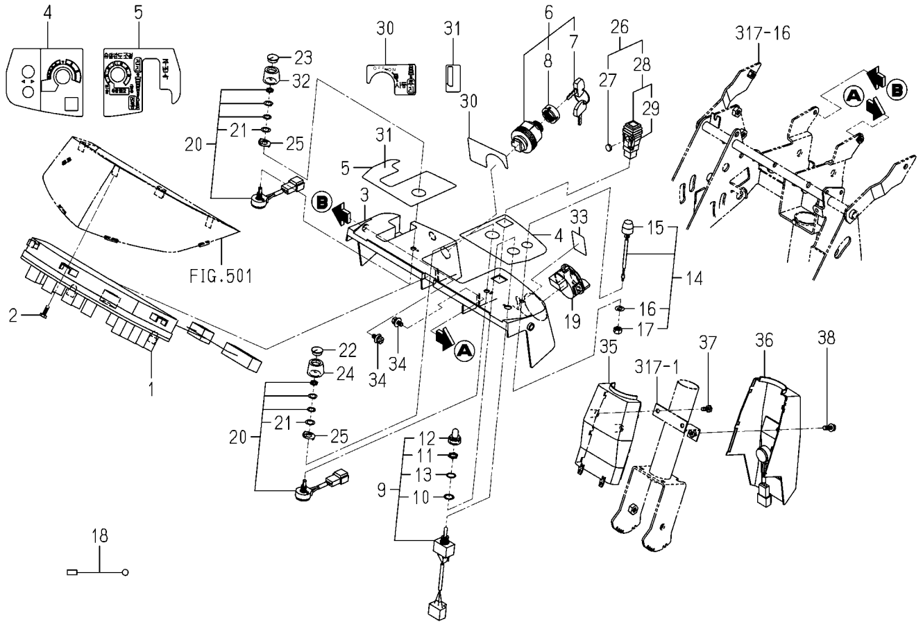
FIG.521 PANEL(MONITOR)SYSTEM(D TYPE)
