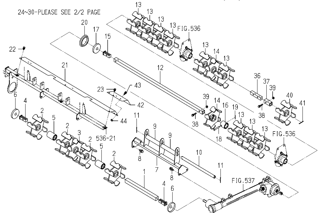
FIG.535 ROTOR SYSTEM(1/2)
