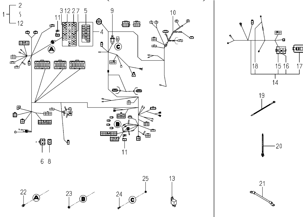
FIG.524 HARNESS(TRAVELING SECTION)SYSTEM (D TYPE EXCEPT F)
