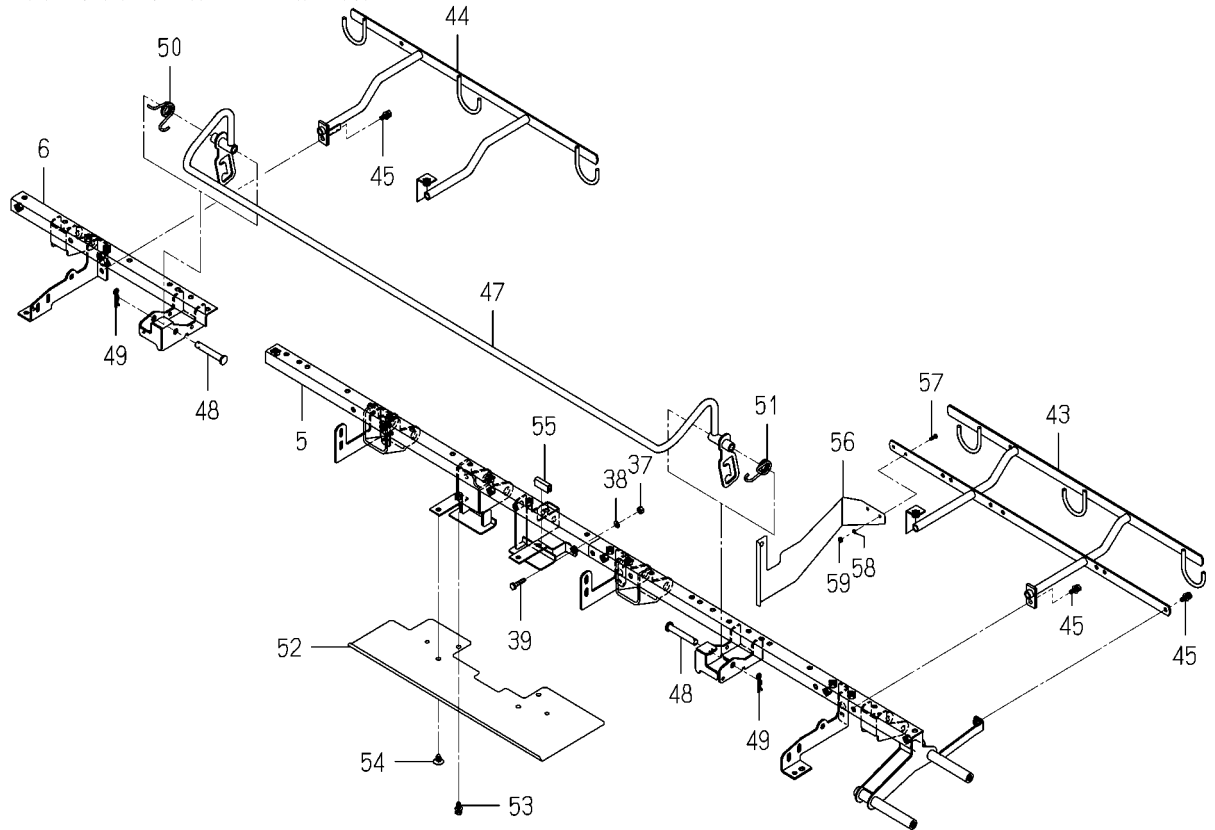
FIG.E08 FRAME(FERTILIZER)SYSTEM(2/2) (DF TYPE)
