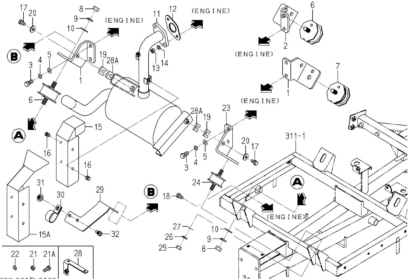
FIG.103 BRACKET(ENGINE)SYSTEM(D TYPE)
