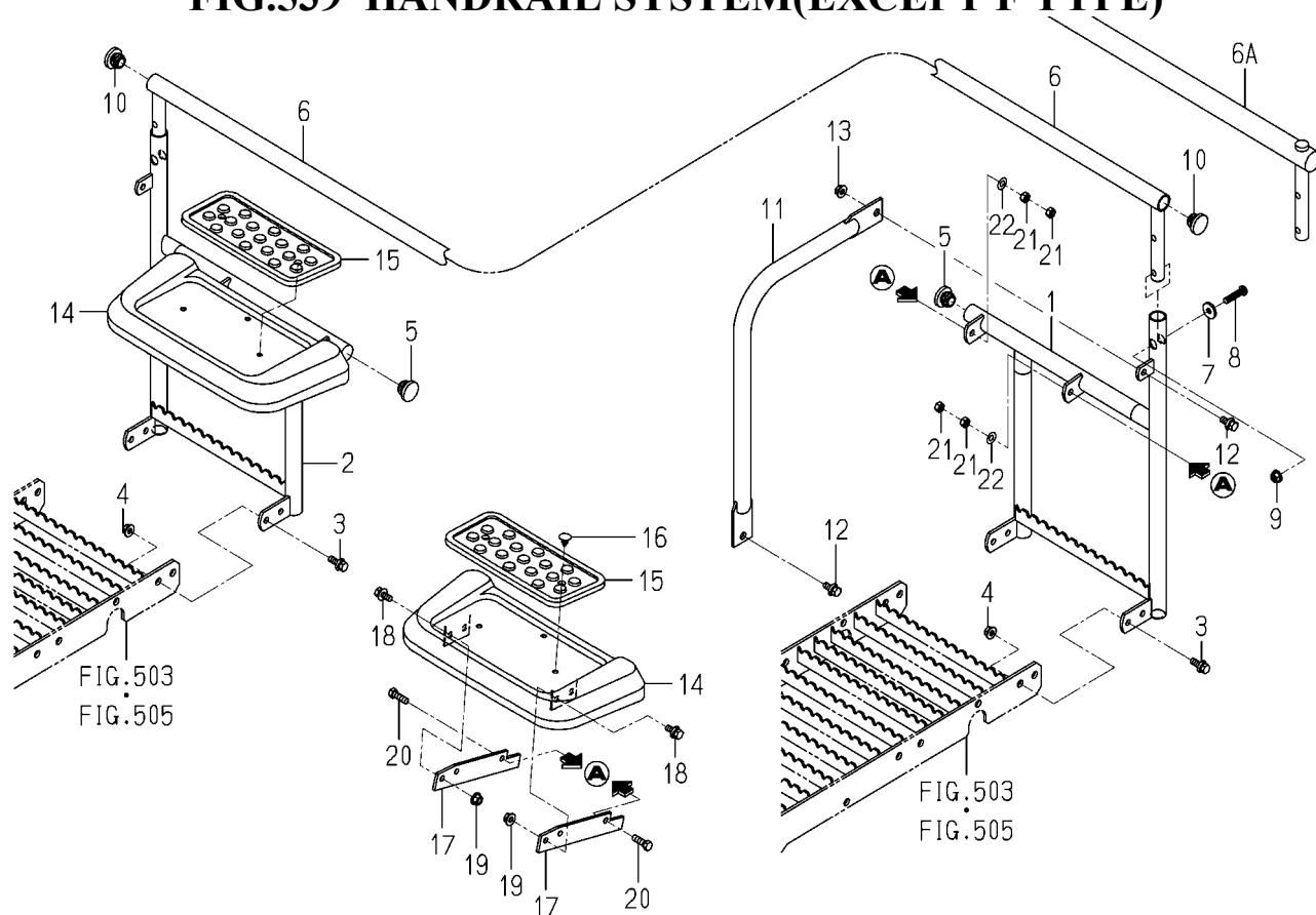
FIG.539 HANDRAIL SYSTEM(EXCEPT F TYPE)
