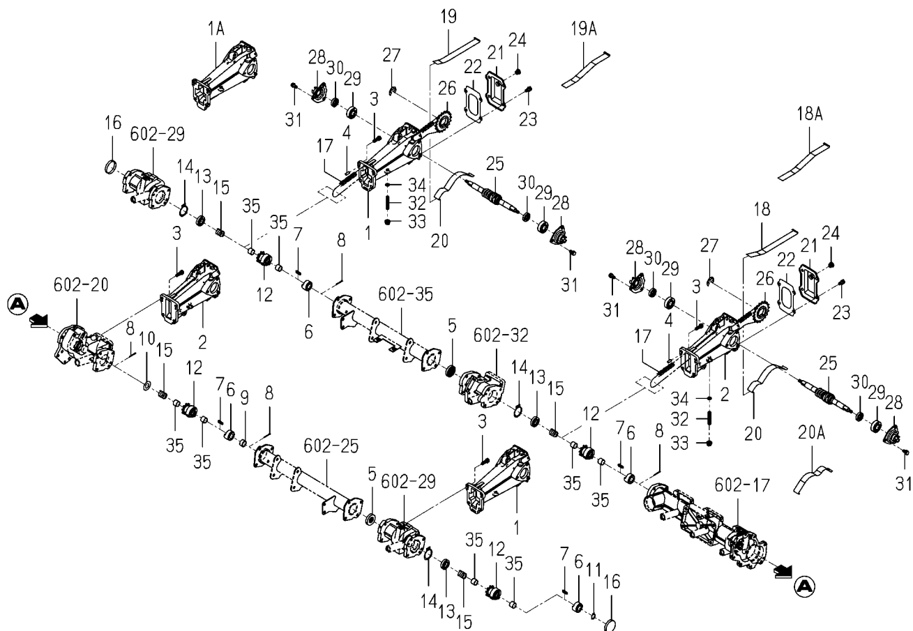
FIG.701 FRAME(SIDE)SYSTEM
