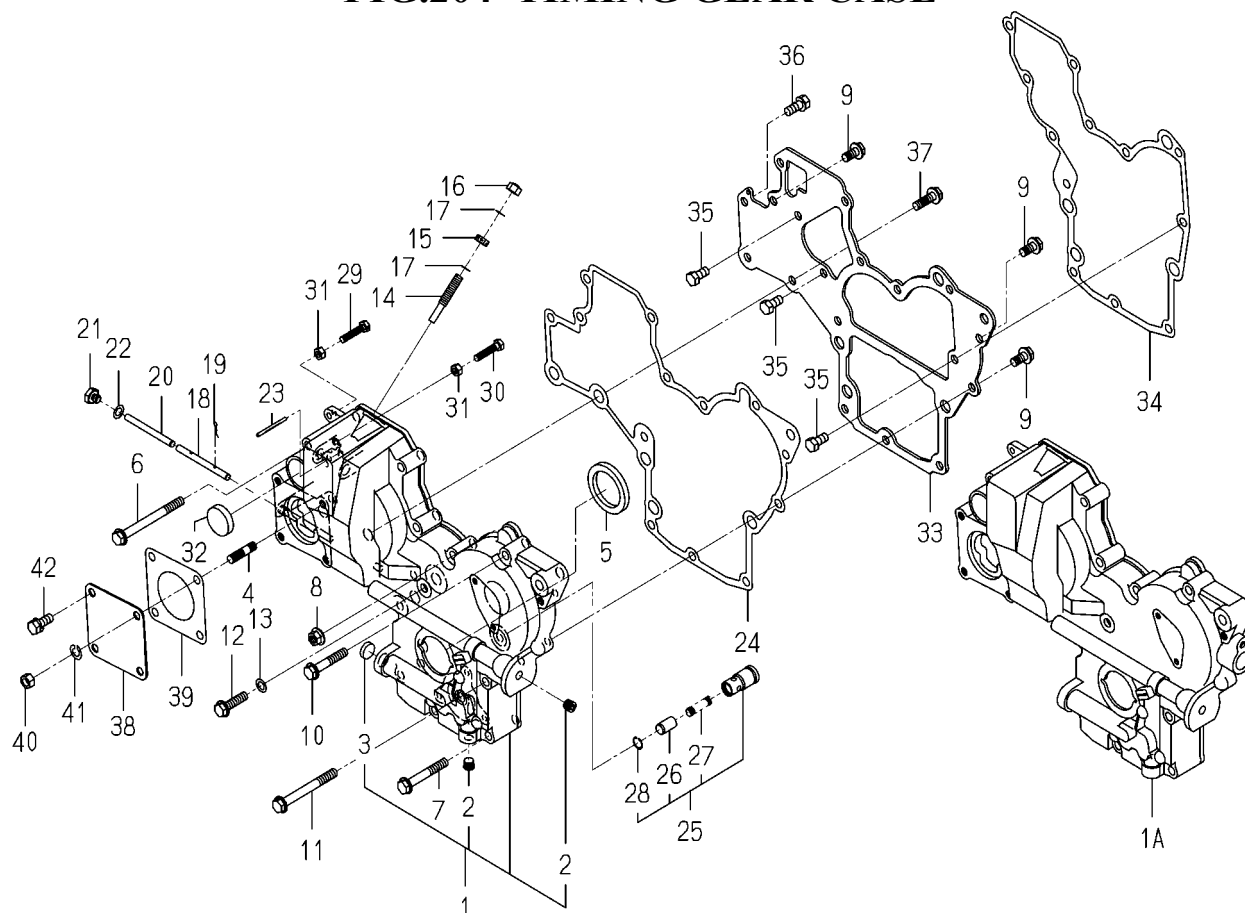
FIG.204 TIMING GEAR CASE
