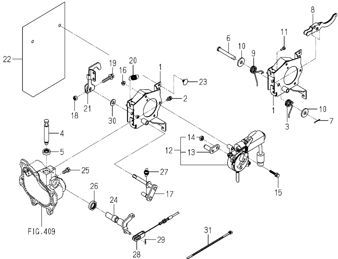
FIG.412 MOTOR(PLANTING)SYSTEM(F TYPE)
