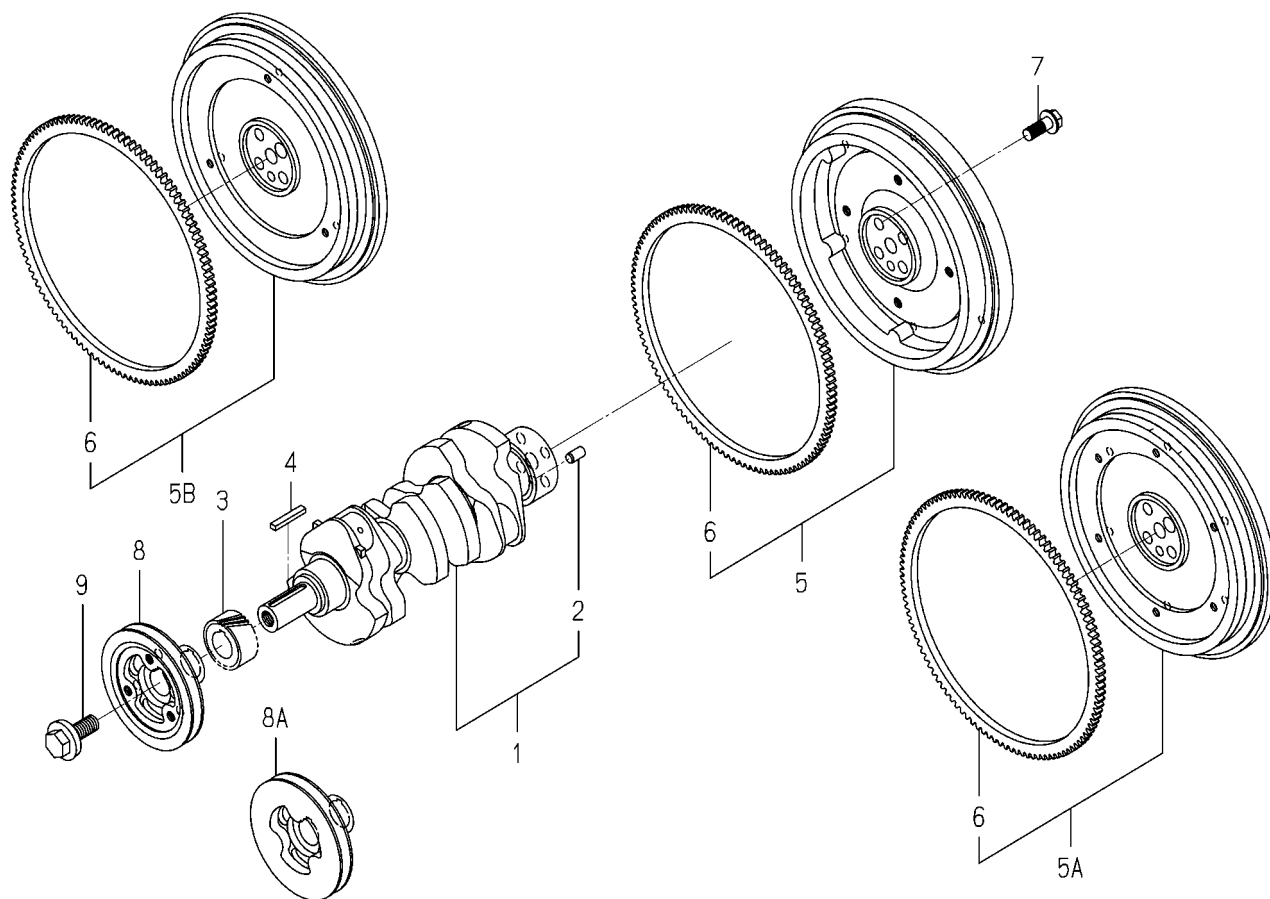
FIG.304 CRANK SHAFT
