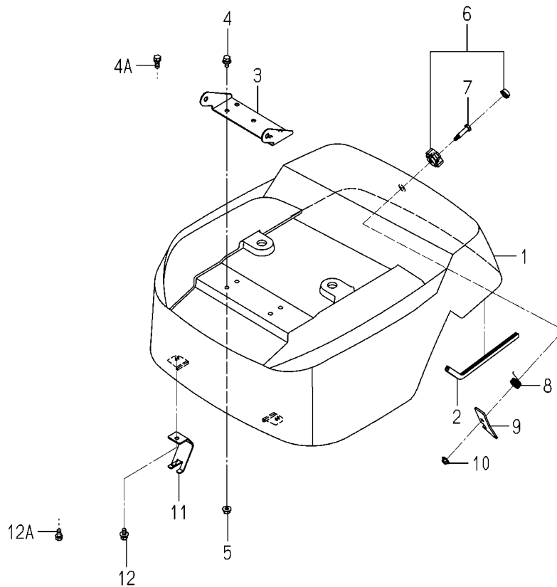
FIG.511 COVER(ENGINE)SYSTEM(D TYPE)
