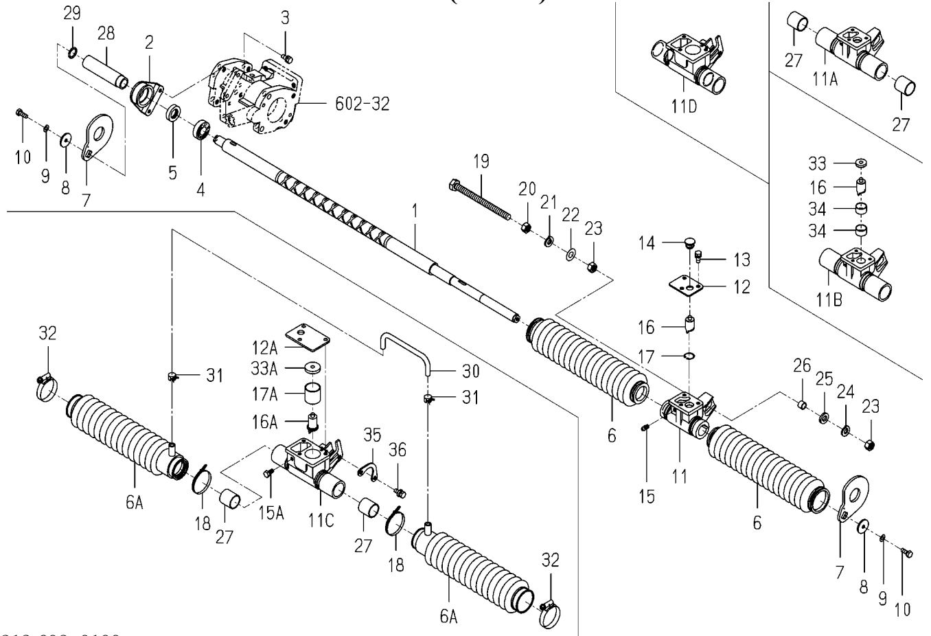
FIG.605 CAM(LEAD)SYSTEM
