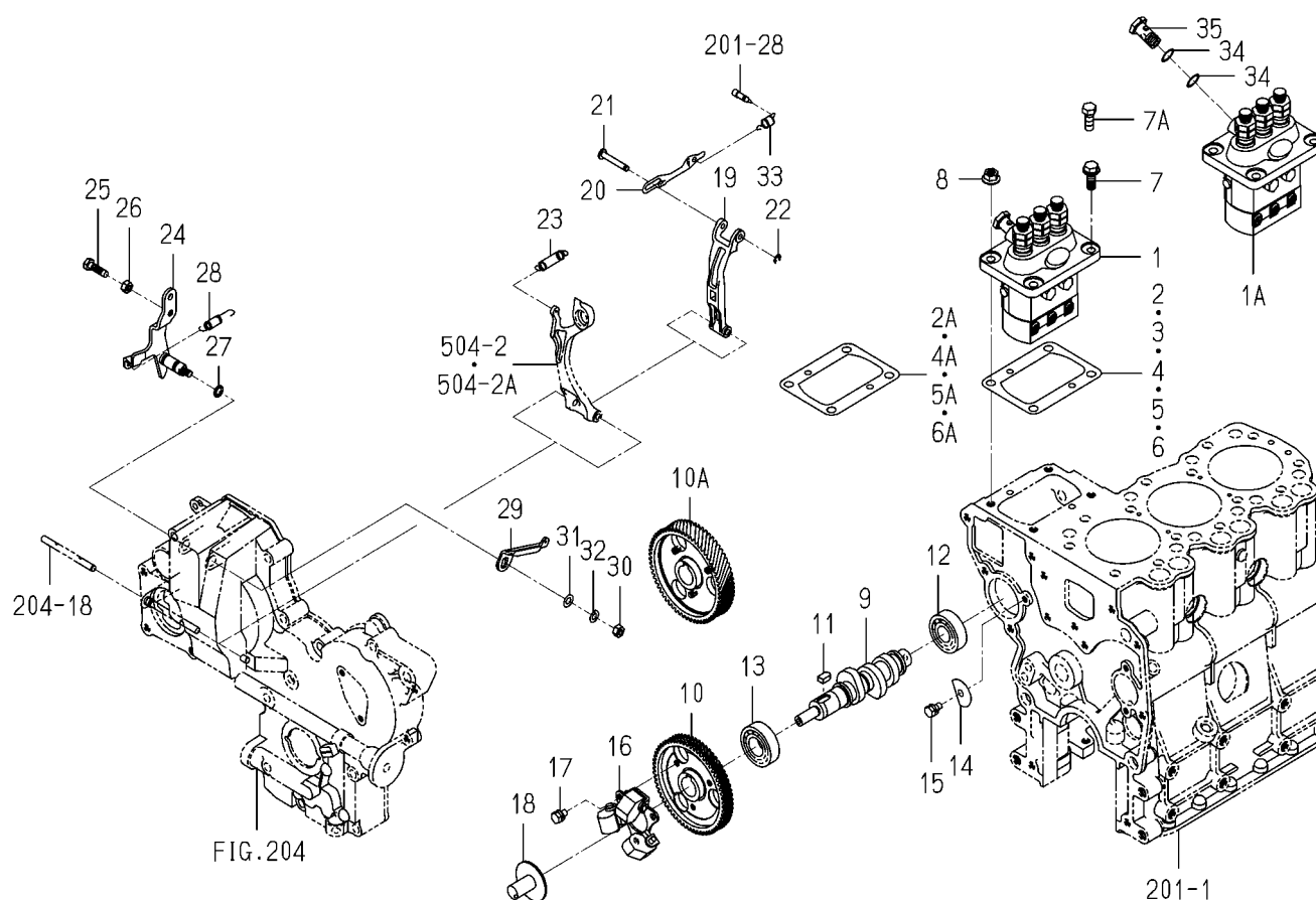
FIG.502 INJECTION PUMP
