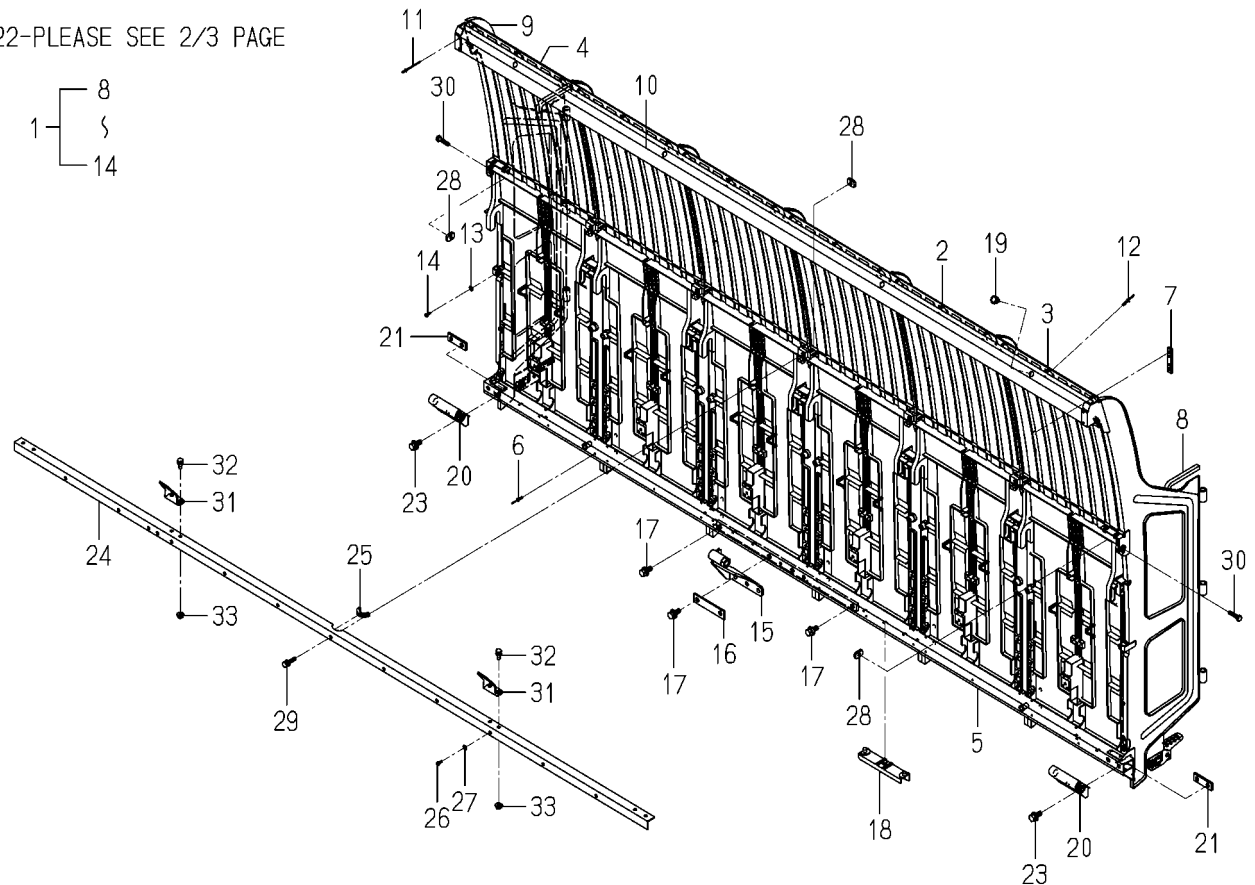
FIG.801 TANK(SEEDLING)SYSTEM(1/3)
