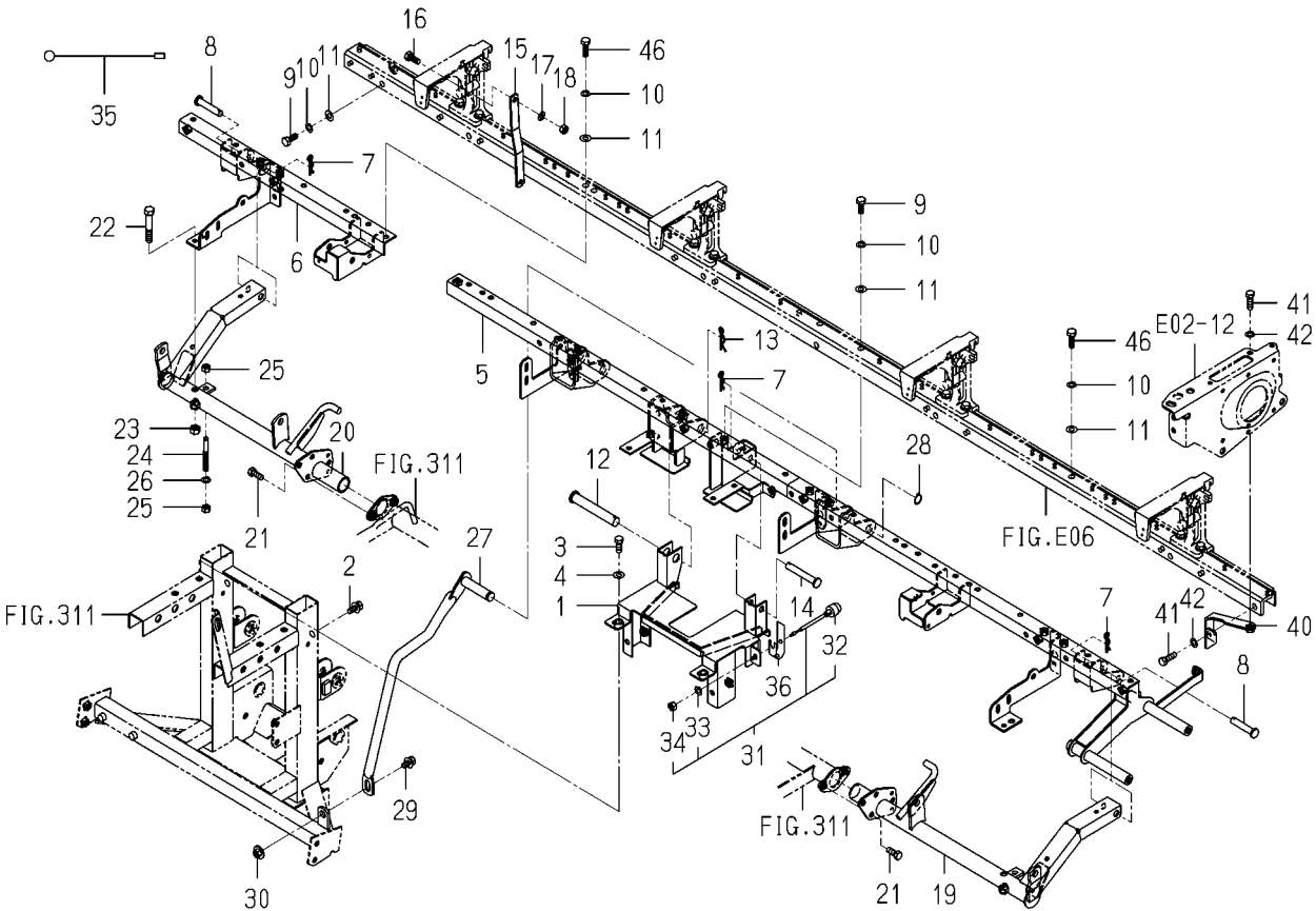
FIG.E08 FRAME(FERTILIZER)SYSTEM(1/2) (DF TYPE)
