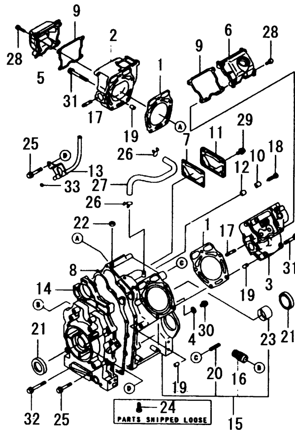
FIG. 1 CYLINDER/CRANKCASE
