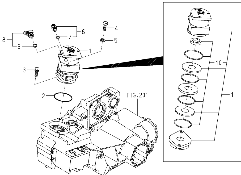
FIG.416 POWER ASSIST(STEERING)SYSTEM
