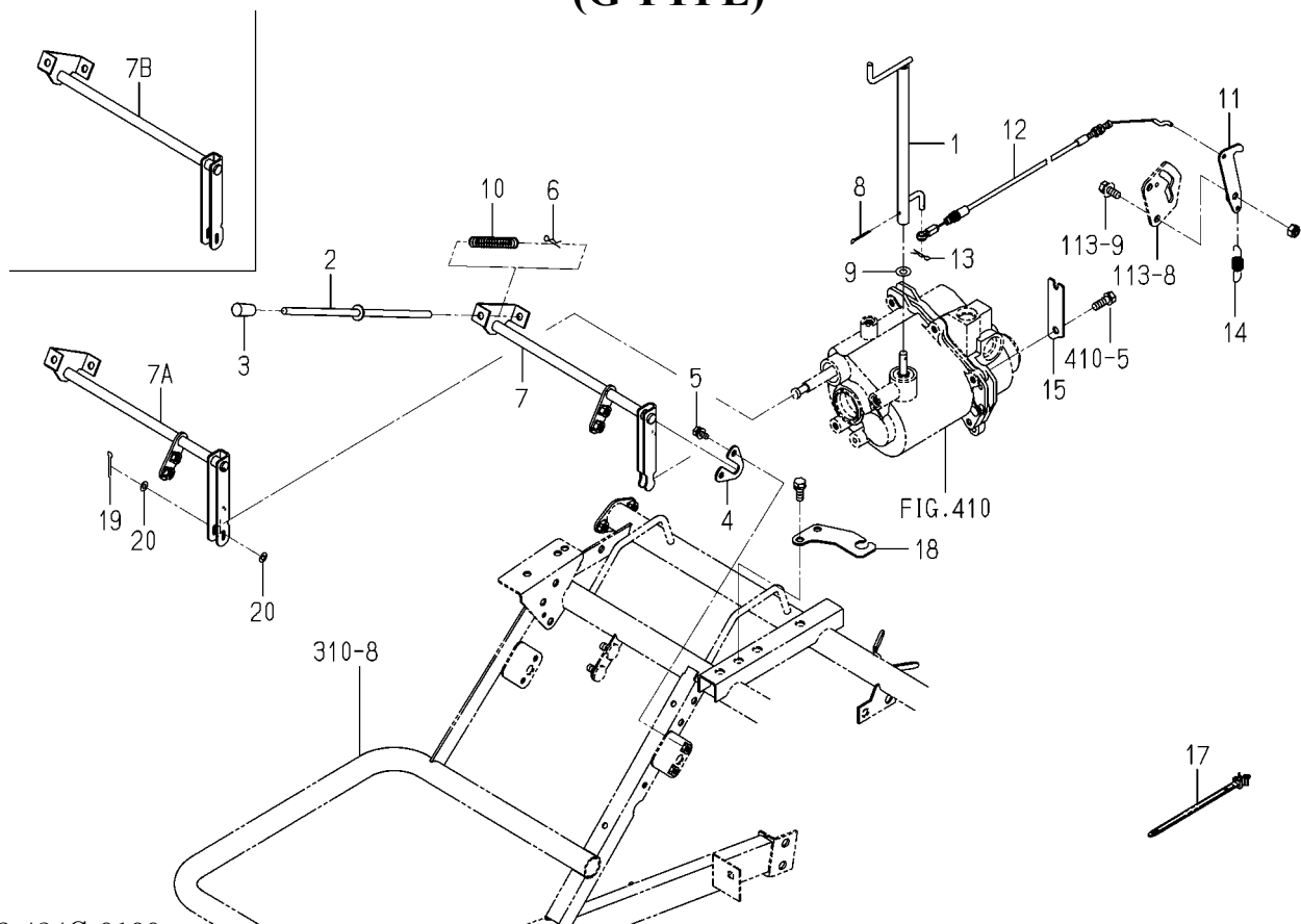
FIG.414 LEVER(PLANTING INTERVAL)SYSTEM (G TYPE)
