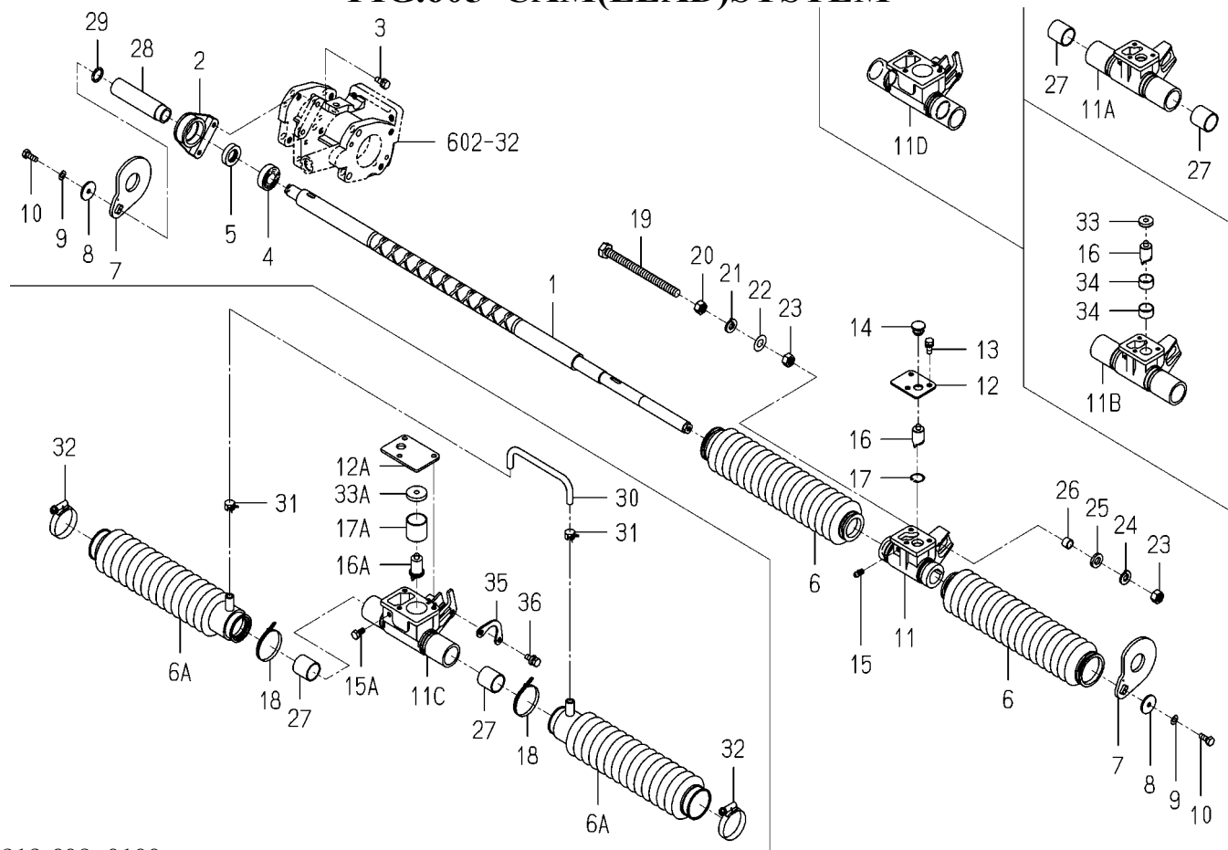
FIG.605 CAM(LEAD)SYSTEM
