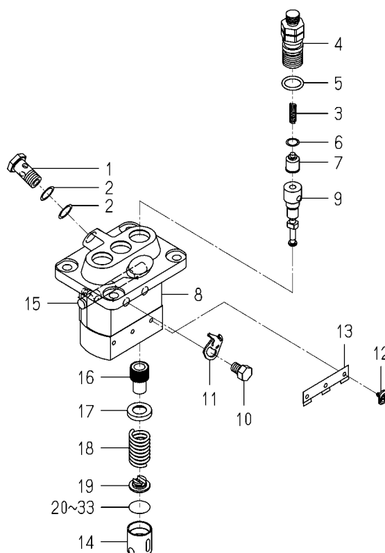
FIG.S02 COMPONENT PARTS FOR 6215-600-103-30 ON Fig.502
