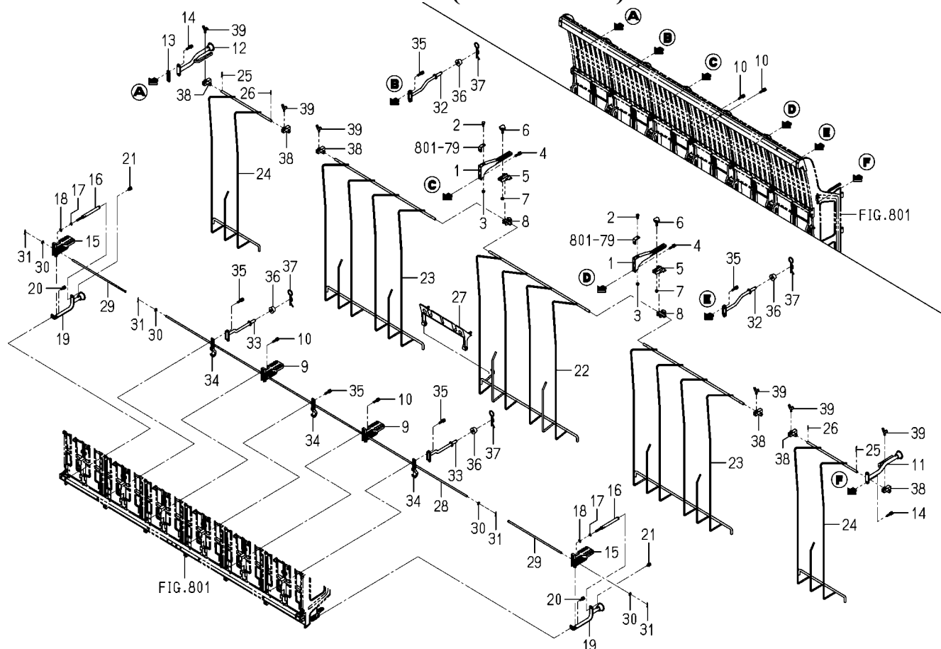
FIG.804 HOLDER(SEEDLING)SYSTEM
