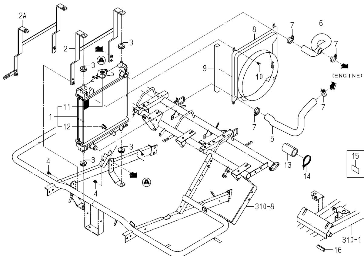
FIG.106 RADIATOR&CLEANER(AIR)SYSTEM (G TYPE)
