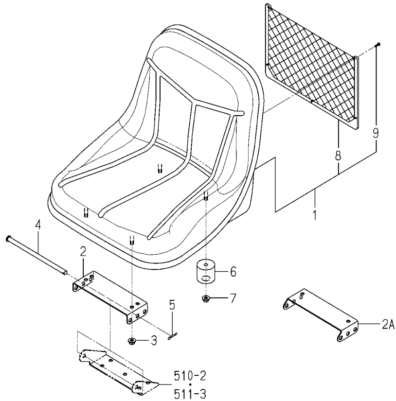
FIG.515 SEAT SYSTEM
