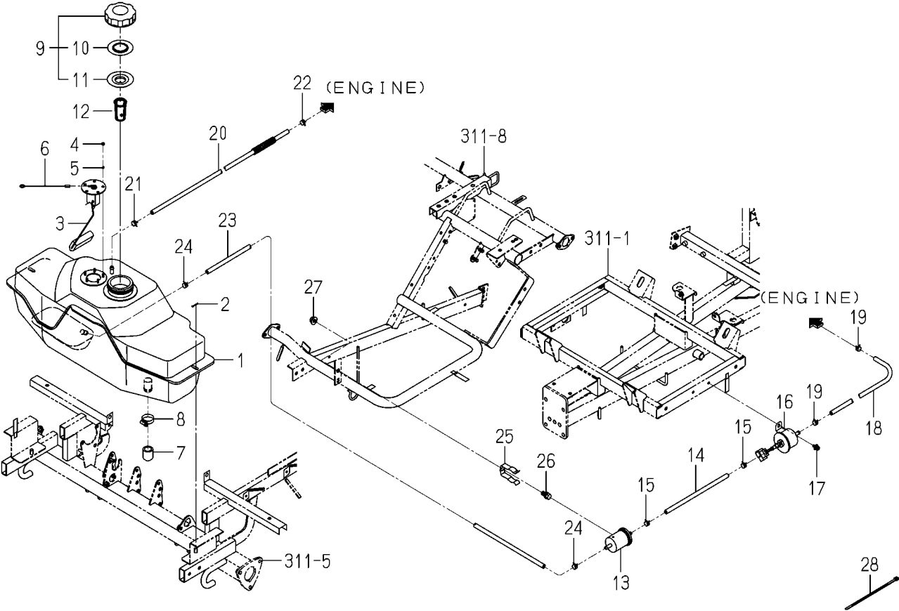
FIG.111 TANK(FUEL)SYSTEM(D TYPE)
