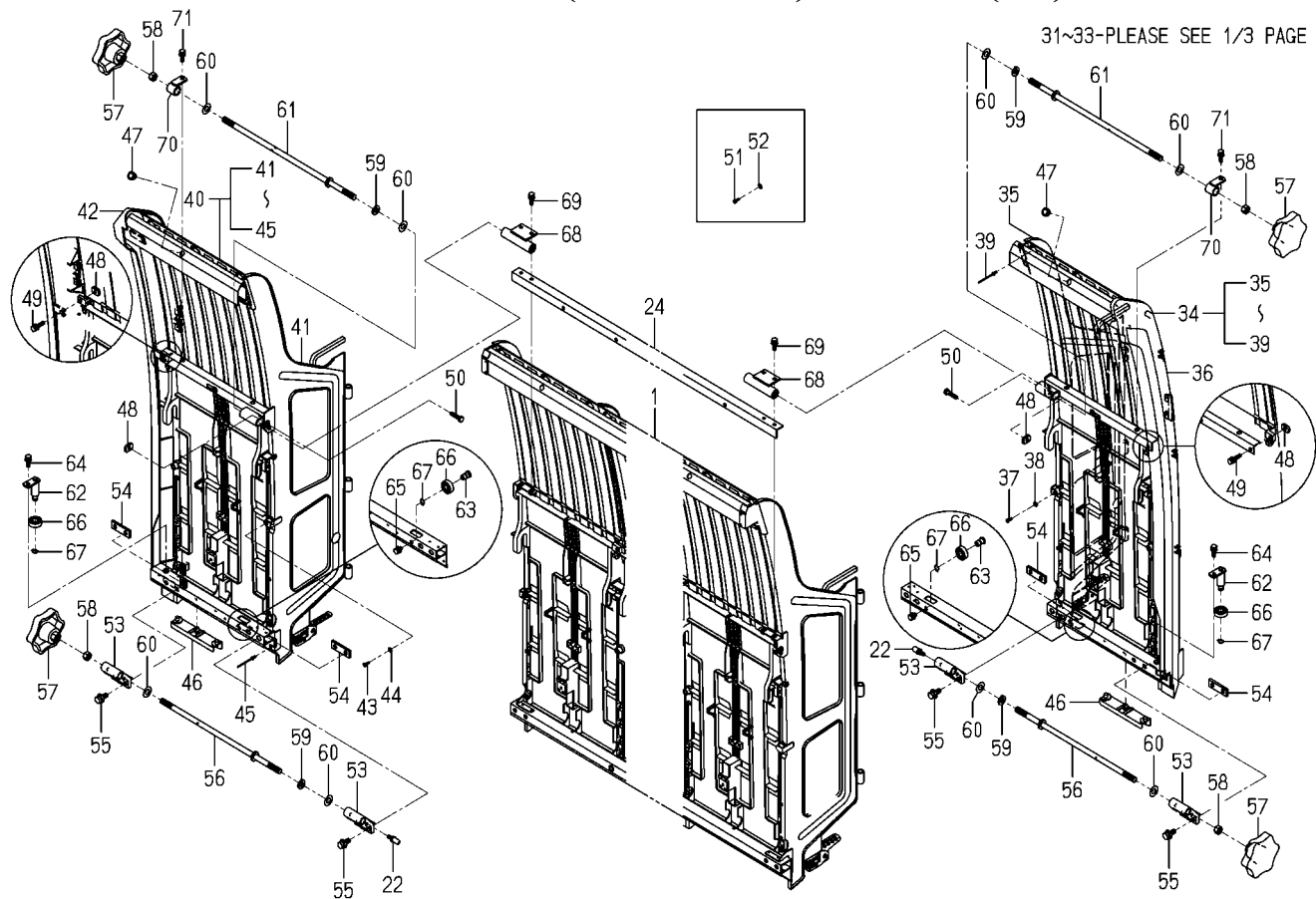
FIG.801 TANK(SEEDLING)SYSTEM(2/3)
