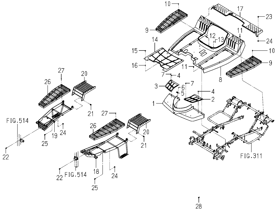
FIG.504 STEP(MAIN)SYSTEM(DF TYPE)
