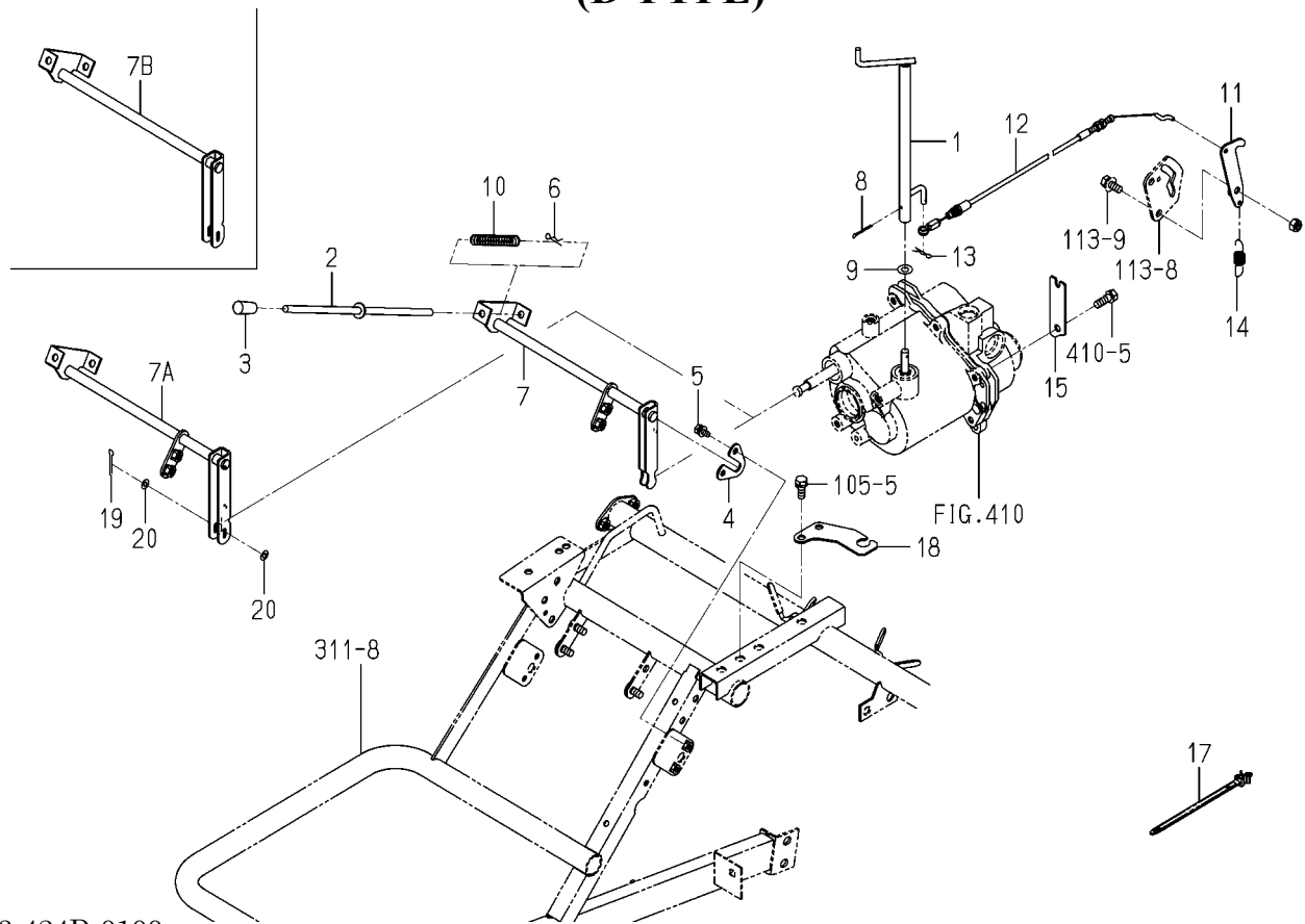
FIG.413 LEVER(PLANTING INTERVAL)SYSTEM (D TYPE)
