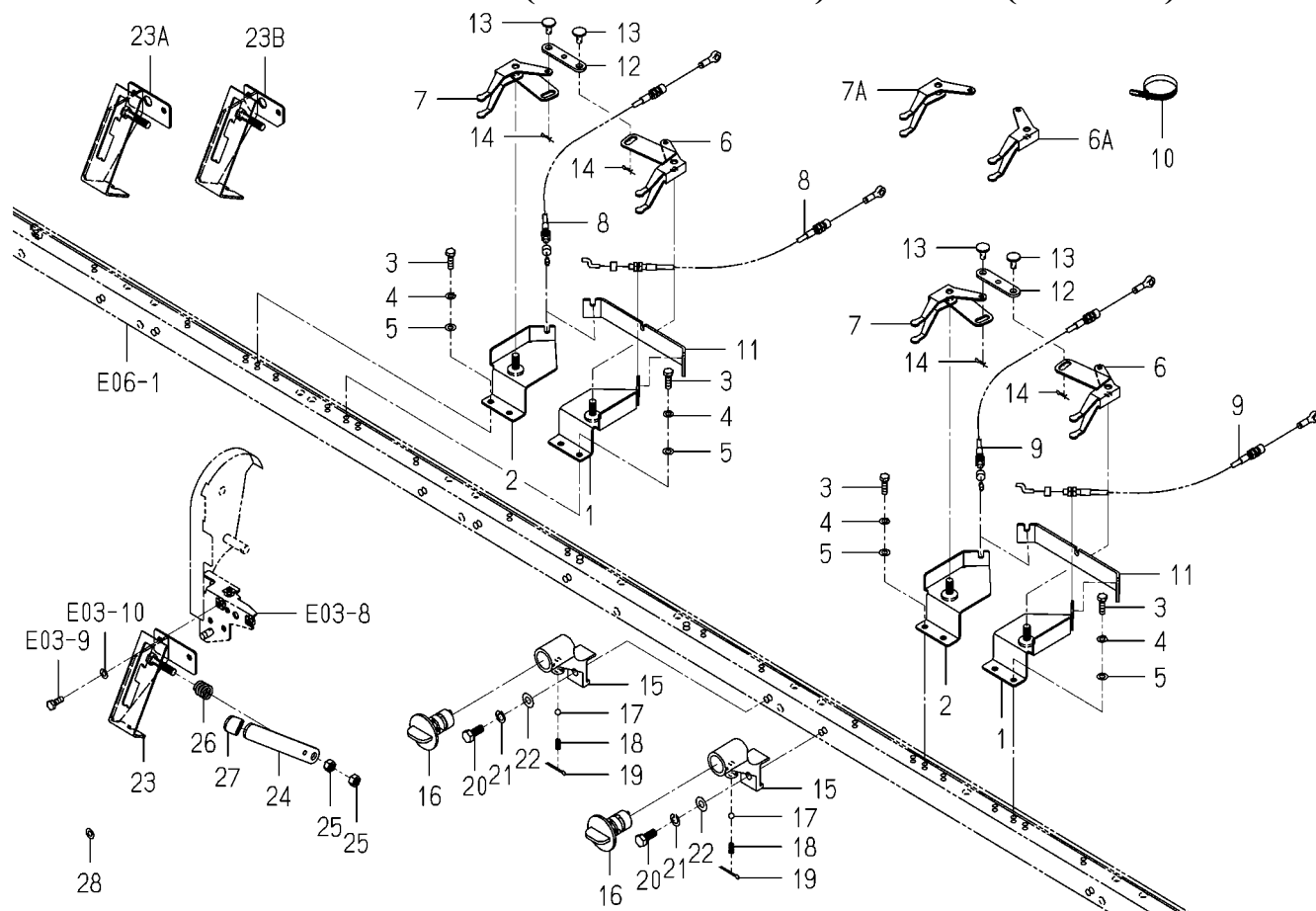
FIG.E14 CLUTCH(FERTILIZING)SYSTEM(F TYPE)
