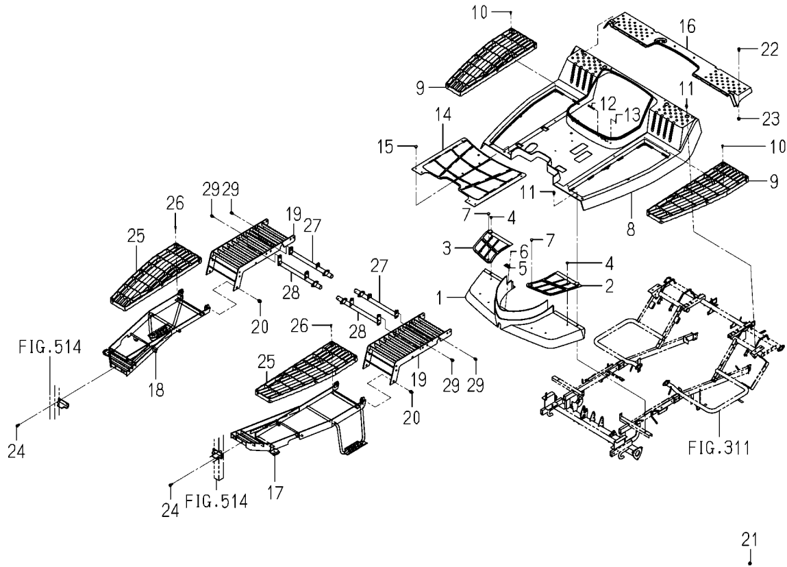
FIG.503 STEP(MAIN)SYSTEM(D TYPE EXCEPT F)
