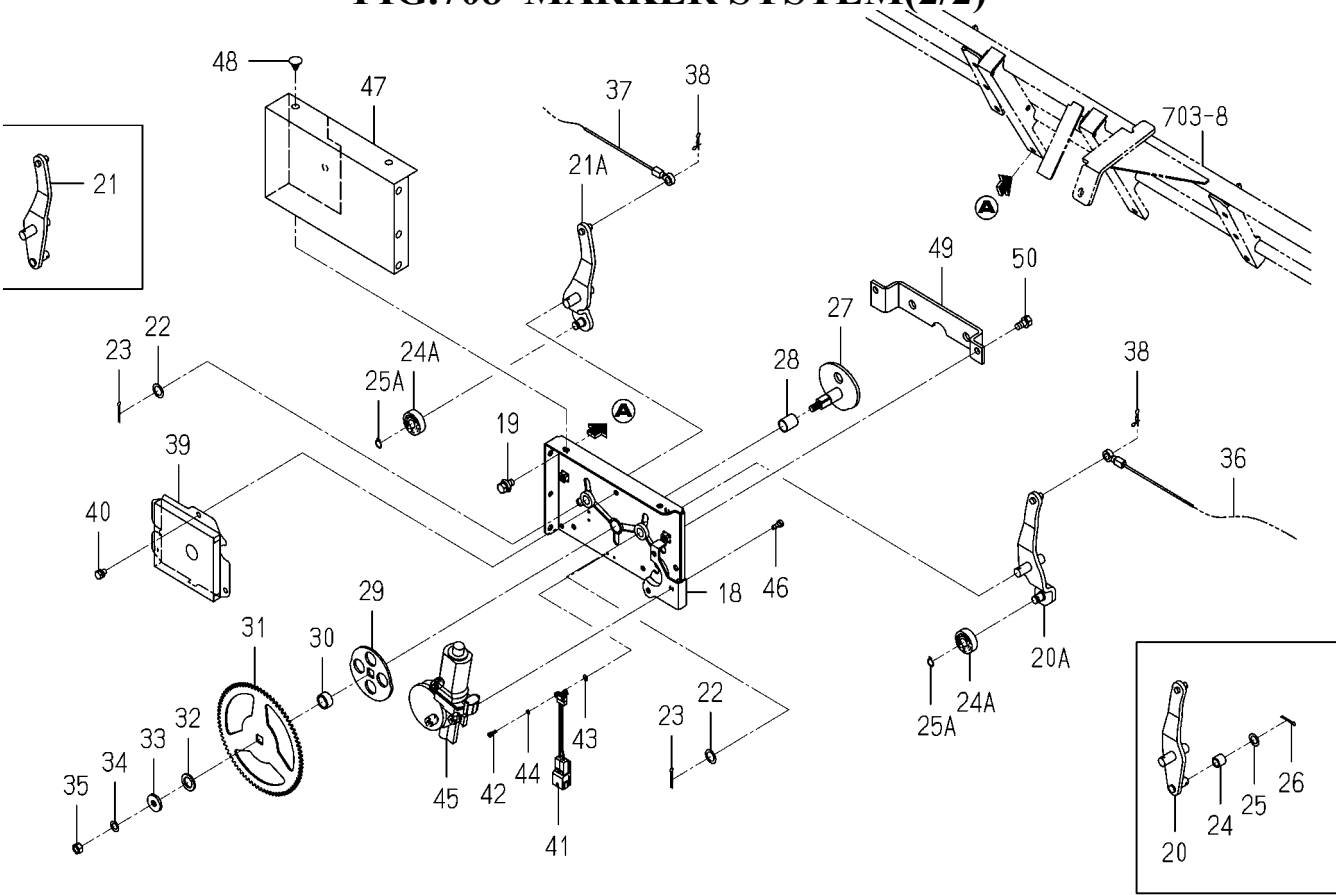
FIG.708 MARKER SYSTEM(2/2)
