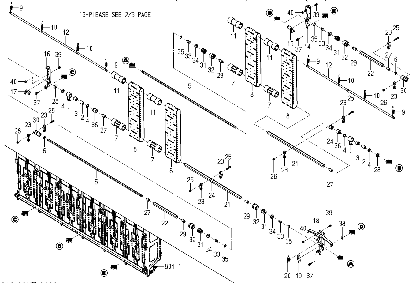
FIG.805 FEED(SEEDLING)SYSTEM(1/3)
