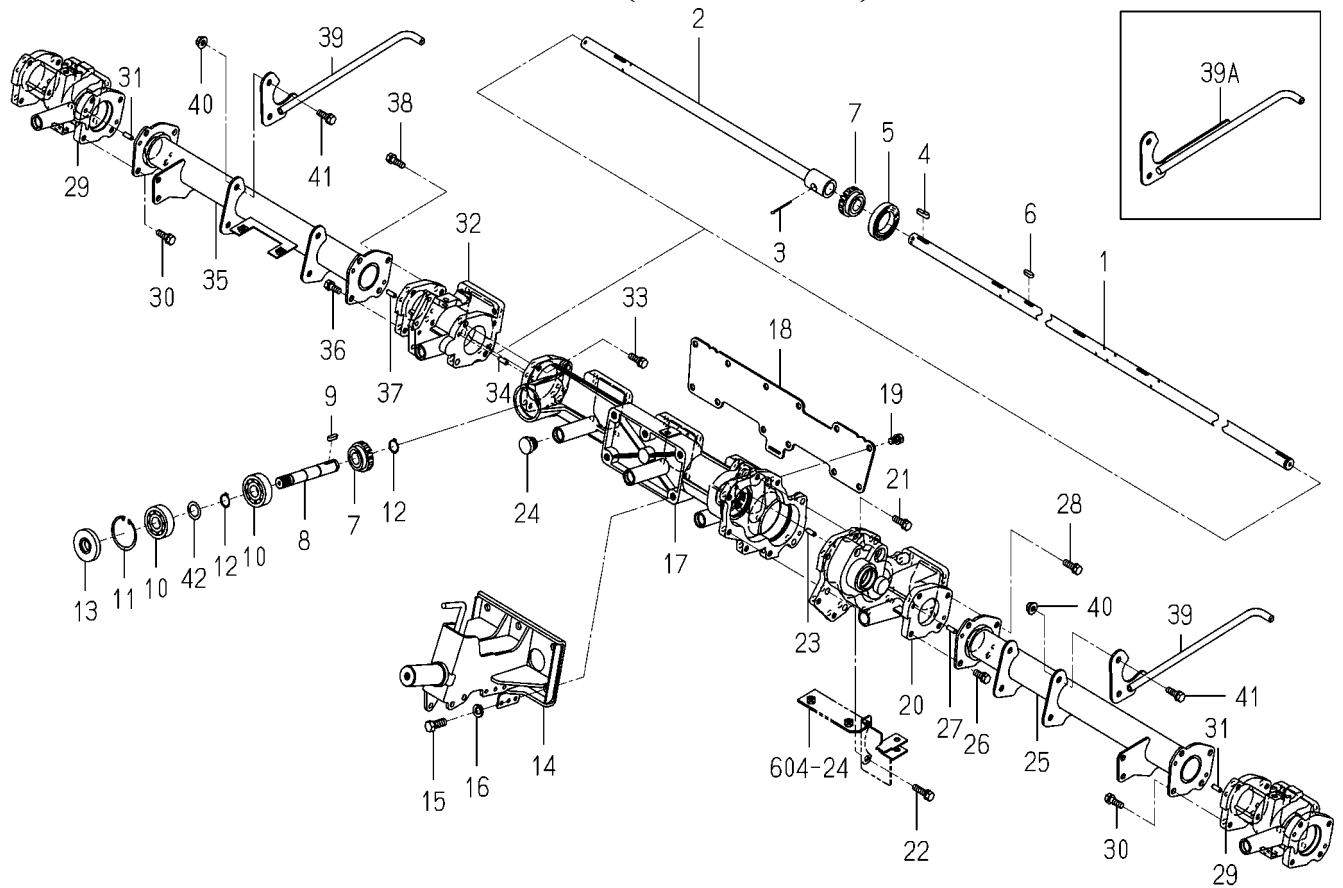
FIG.602 FRAME(PLANTING)SYSTEM
