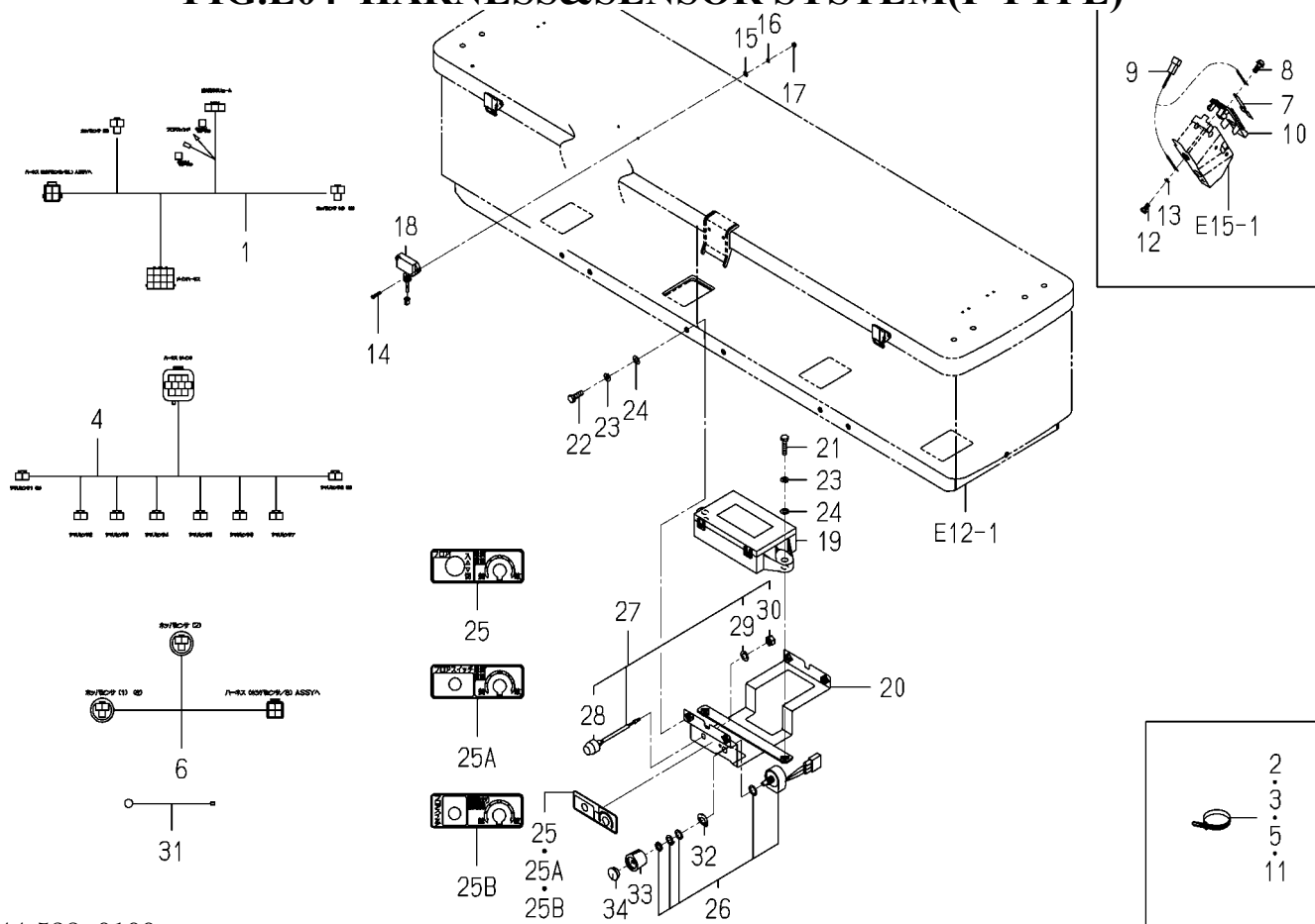
FIG.E04 HARNESS&SENSOR SYSTEM(F TYPE)
