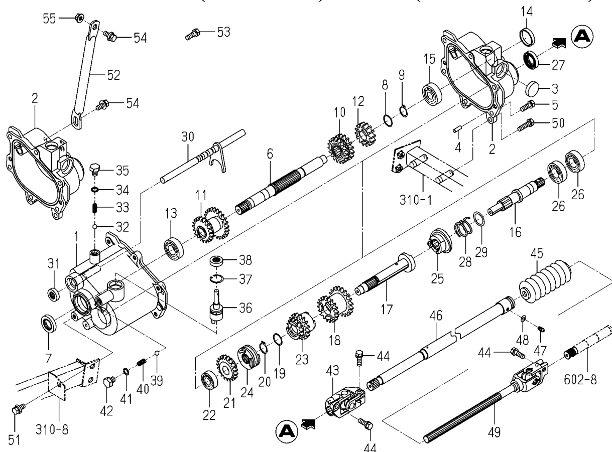
FIG.410 CASE(PLANTING)SYSTEM(EXCEPT F TYPE)
