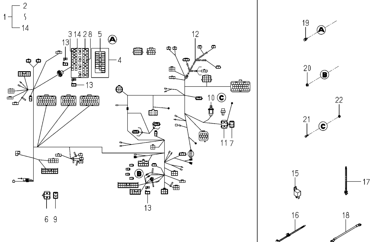
FIG.523 HARNESS(TRAVELING SECTION)SYSTEM (GF TYPE)
