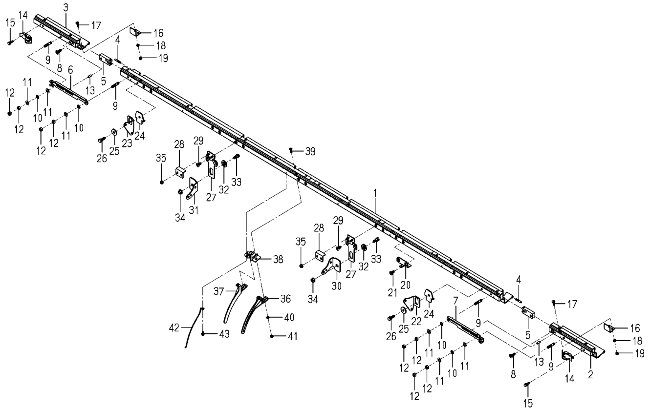
FIG.803 PLATE(FRONT)SYSTEM
