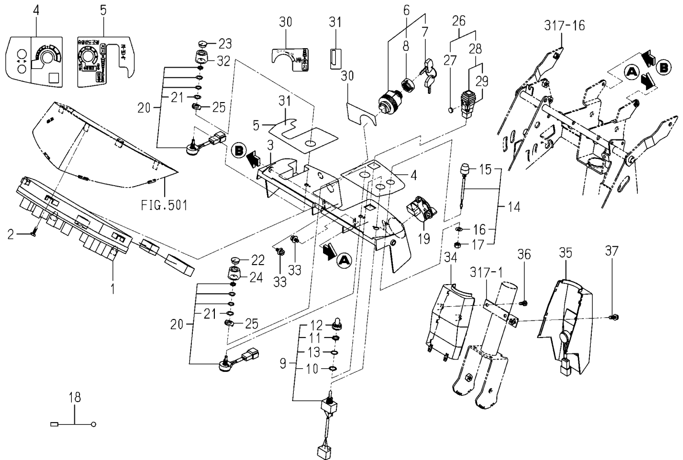
FIG.520 PANEL(MONITOR)SYSTEM(G TYPE)
