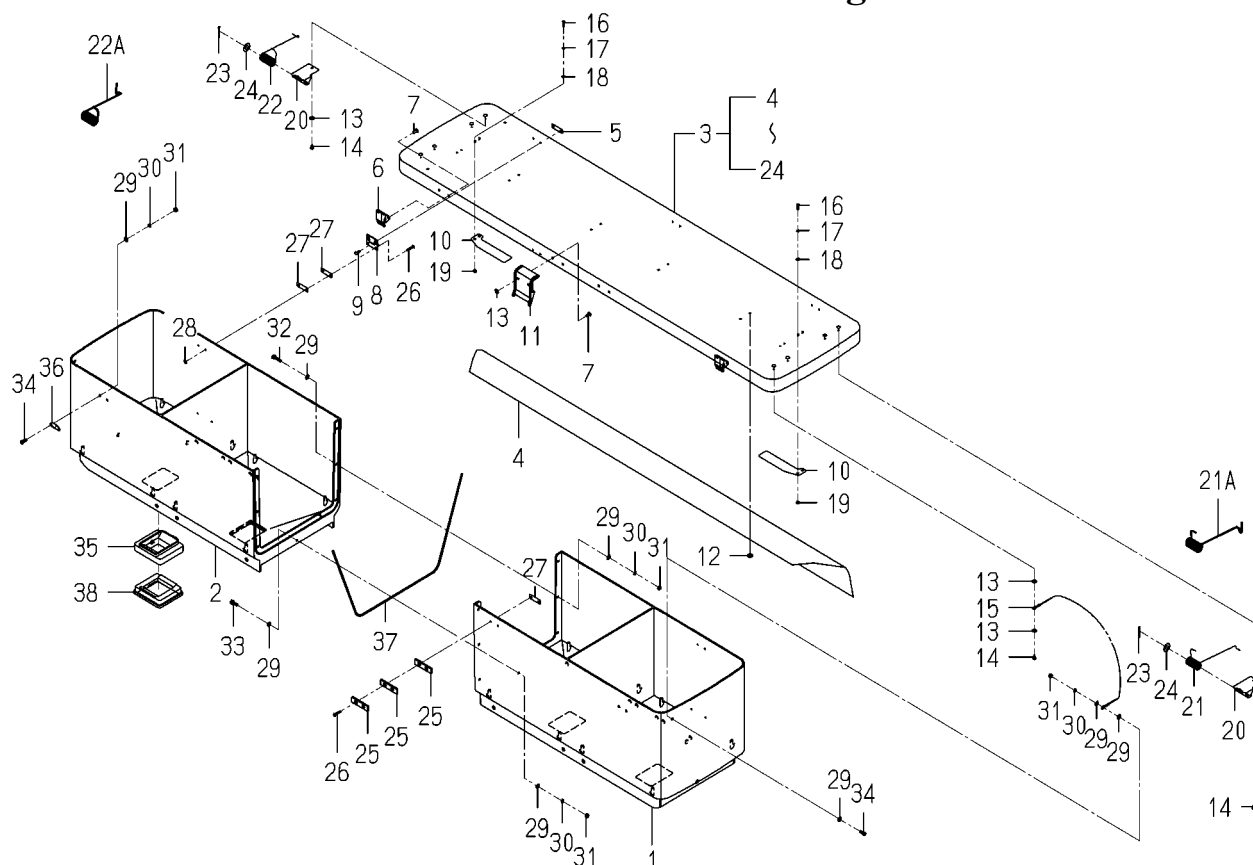
FIG.S06 COMPONENT PARTS FOR 8844-718-310-40 ON Fig.E12
