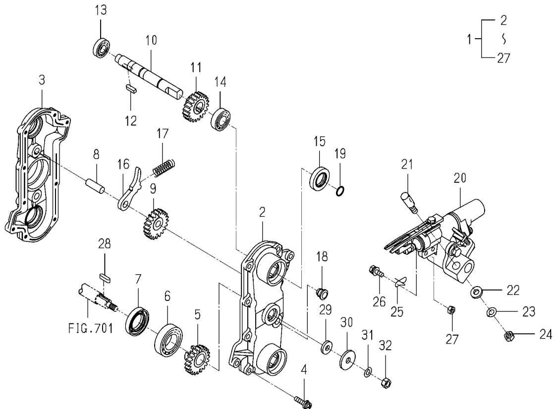
FIG.710 PLANTER(LH)SYSTEM
