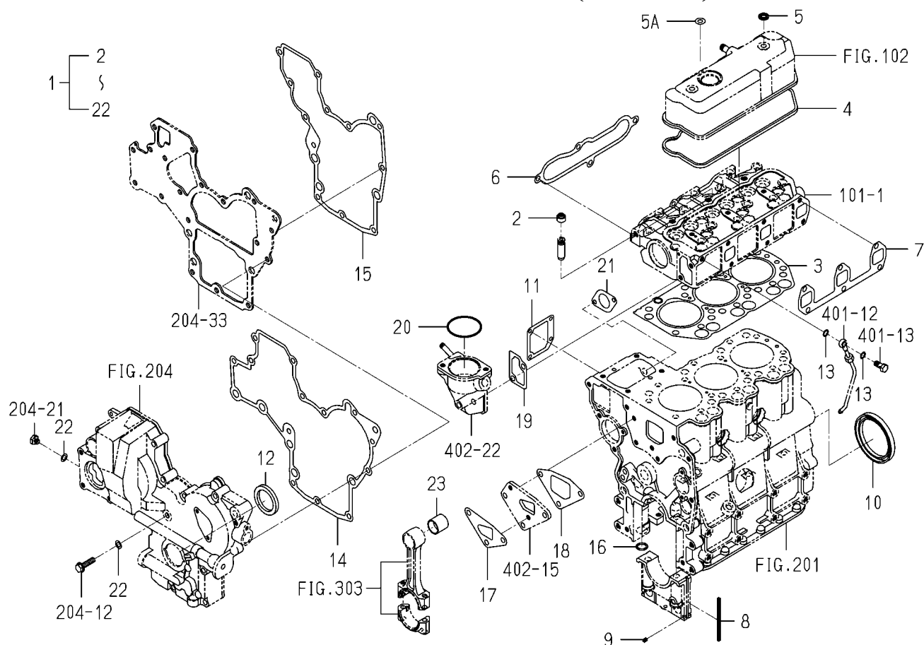
FIG.P03 REPAIR PARTS (OPTION)
