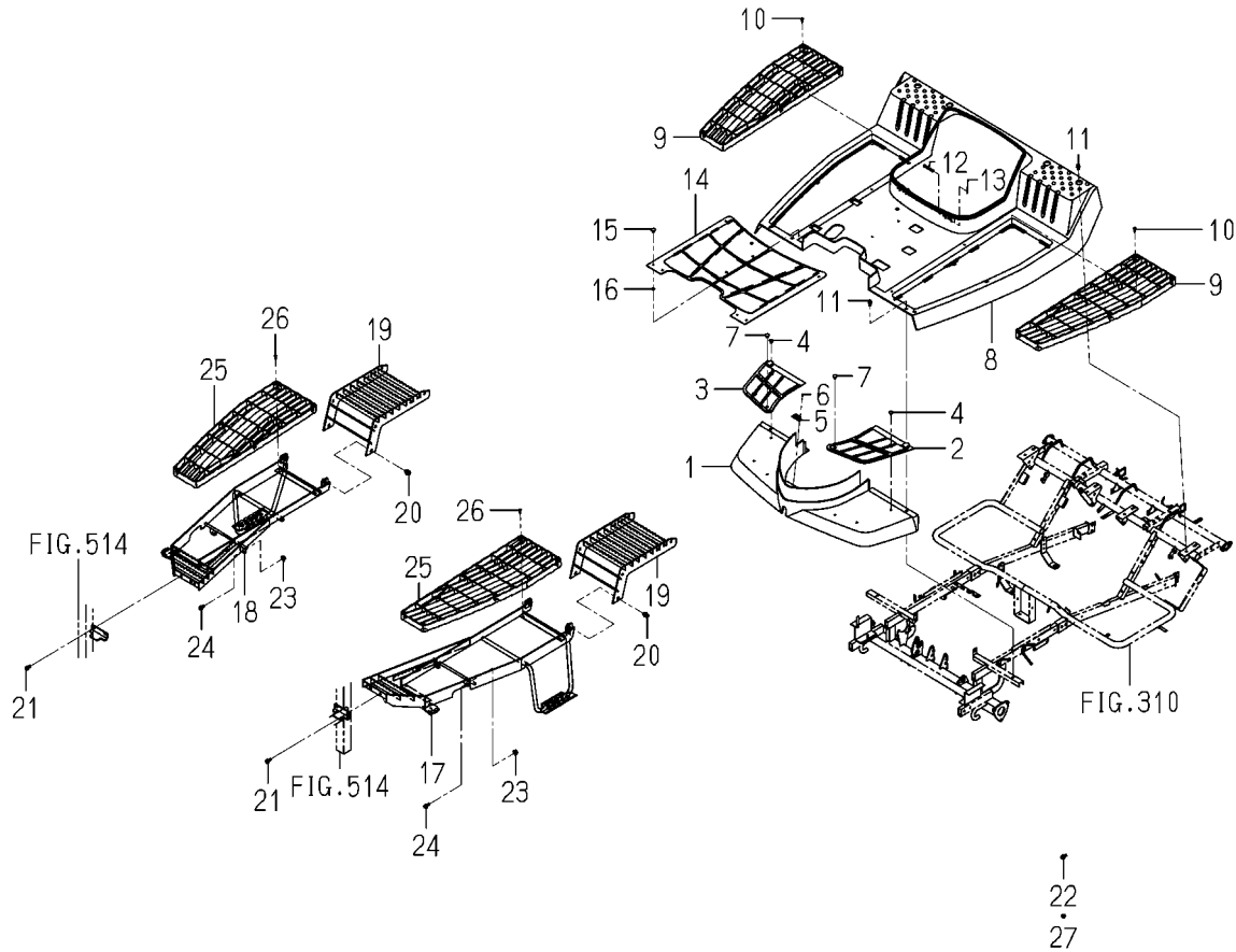
FIG.506 STEP(MAIN)SYSTEM(GF TYPE)
