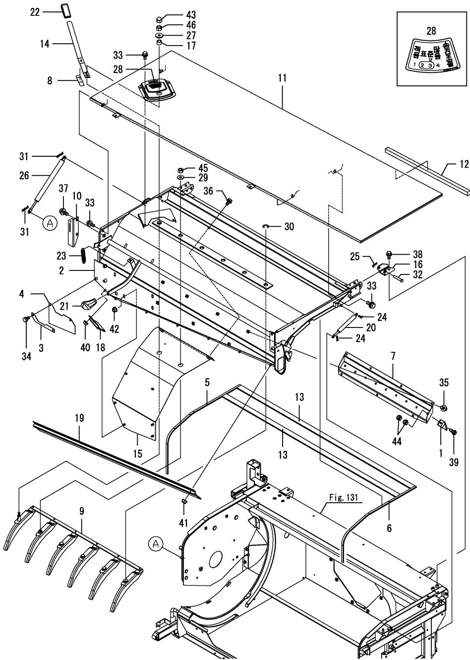
OCNP6-M05021 탈곡(1) Fig.164. 탈곡실커버
